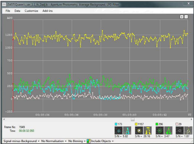
Figure 7: Station 1 Tangra lightcurves, exposure time 60 ms, target star cyan.
