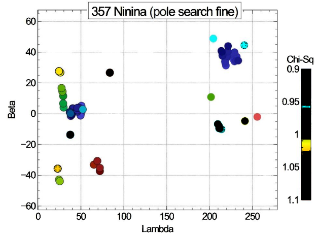
Figure 6: The “fine” pole search shows two clustered solutions (dark blue color) approximately centered near ecliptic longitude-latitude pairs (50^\circ, 3^\circ) and (228^\circ, 35^\circ) with a radius of 10^\circ and Chi-Sq values within 10% of the lowest value.
