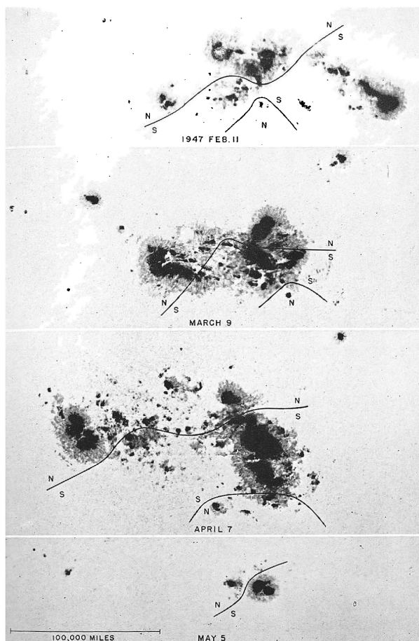
Figure 18. Mt Wilson photographs of groups 14813, 14851, 14886 & 14933 (1947 February to May). 29
