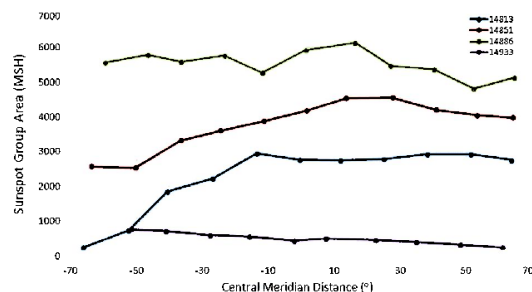
Figure 19. Greenwich sunspot area for groups 14813, 14851, 14886 & 14933 (1947 February to May).
