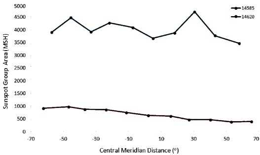
Figure 12. Greenwich sunspot area for groups 14585 & 14620 (1946 July and August).
