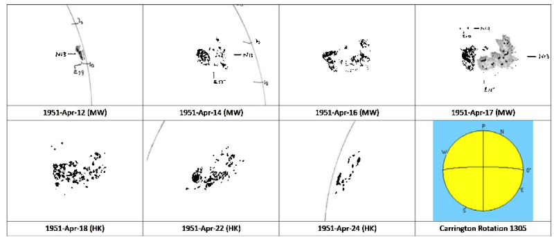
Figure 22. Passage of Greenwich group 16745, based on Mt Wilson (MW) and Hisako Koyama (HK) drawings.
