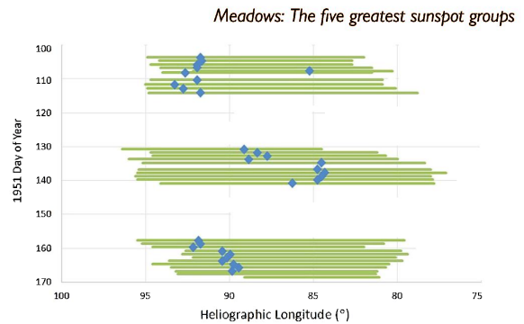
Figure 27. Longitude evolution of group 16763, with previous and subsequent rotations.
