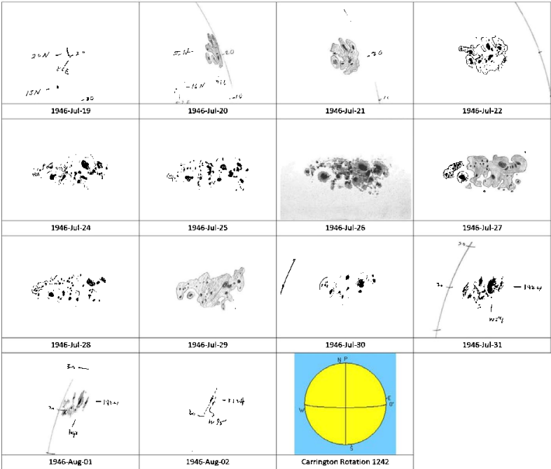
Figure 8. Passage of Greenwich group 14585, based on Mt Wilson drawings and a photograph. 22
