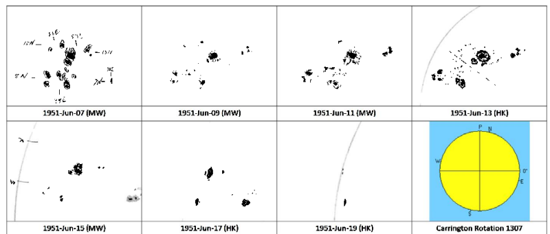
Figure 25. Passage of Greenwich group 16792, based on Mt Wilson (MW) and Hisako Koyama (HK) drawings.
