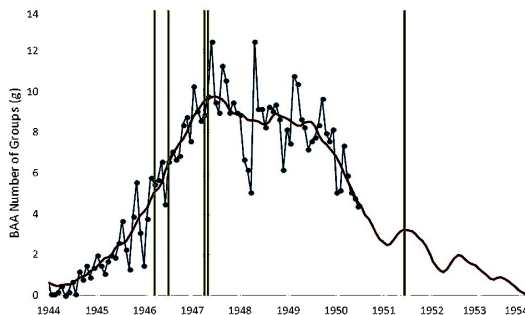
Figure 2. BAA mean daily frequency for the number of groups and dates of the five greatest sunspot groups.
