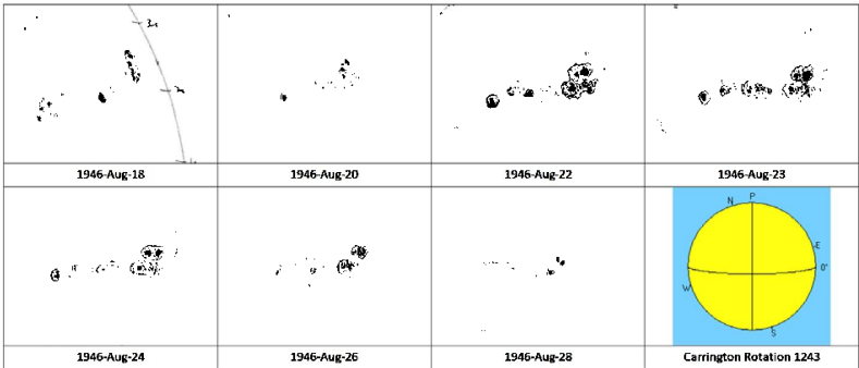
Figure 11. Passage of Greenwich group 14620, based on Mt Wilson drawings.
