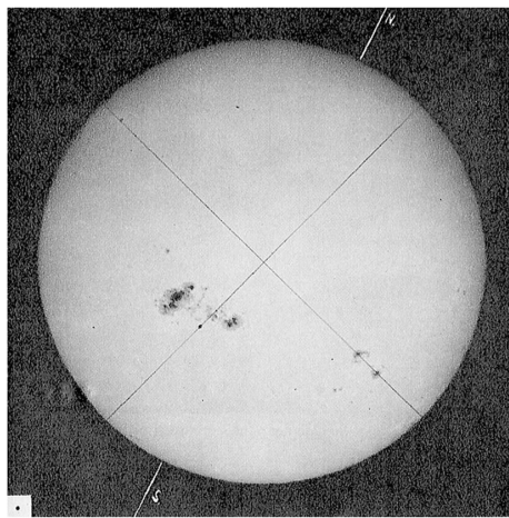
Figure 1. The Great Sunspot of 1947 (Greenwich group number 14886). Photograph from the Royal Observatory, Greenwich, 1947 Apr 7. 7
