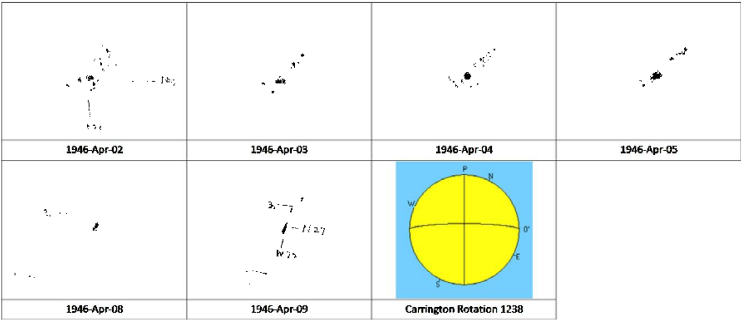
Figure 6. Passage of Greenwich group 14478, based on Mt Wilson drawings.
