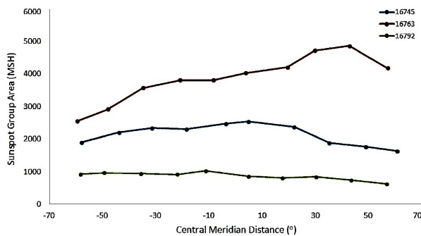
Figure 26. Greenwich sunspot area for groups 16745, 16763 & 16792 (1951 April to June).
