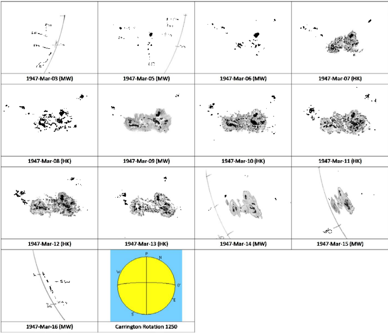
Figure 15. Passage of Greenwich group 14851, based on Mt Wilson (MW) and Hisako Koyama (HK) drawings.
