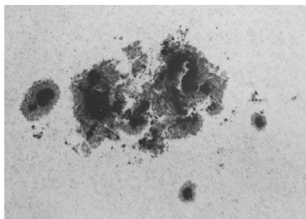
Figure 24. Mt Wilson photograph, taken on 1951 May 17. 30
