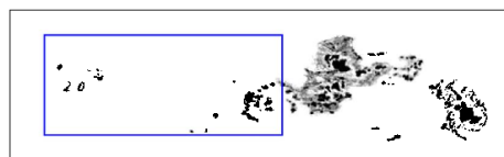
Figure 21. Expected location of groups 14851 & 14886 on 1947 Feb 10 (Hisako Koyama drawing).
