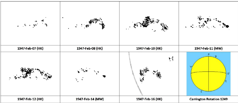
Figure 14. Passage of Greenwich group 14813, based on Mt Wilson (MW) and Hisako Koyama (HK) drawings. 26–28
