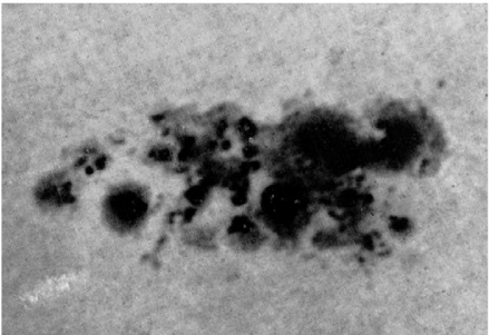
Figure 10. Group 14585 on 1946 Jul 27, by BAA member Mr E. J. Harris. 12
