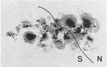
Figure 9. Mt Wilson photograph from 1946 Jul 25. 23
