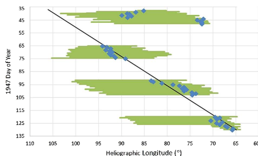
Figure 20. Longitude evolution of groups 14851 & 14886, including previous and subsequent rotations.
