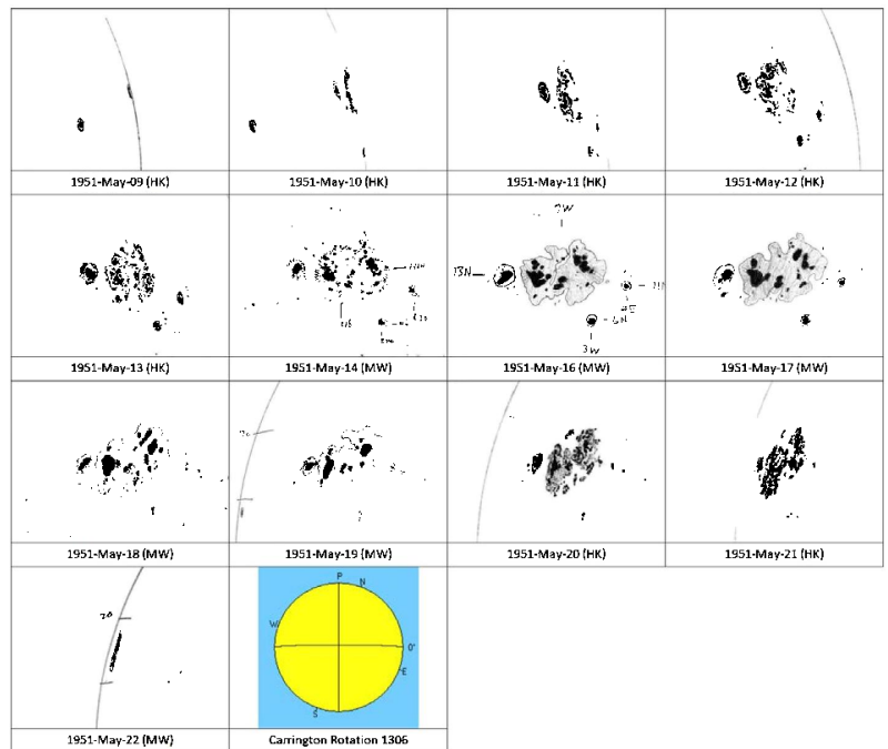
Figure 23. Passage of Greenwich group 16763, based on Mt Wilson (MW) and Hisako Koyama (HK) drawings.
