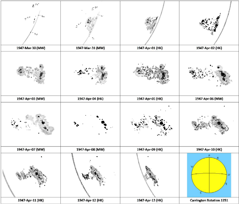
Figure 16. Passage of Greenwich group 14886, based on Mt Wilson (MW) and Hisako Koyama (HK) drawings.
