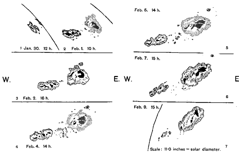
Figure 4. Drawings of the Great Sunspot of 1946 February, by Dr M. A. Ellison. 21
