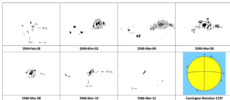
Figure 5. Passage of Greenwich group 14451, based on Mt Wilson drawings.
