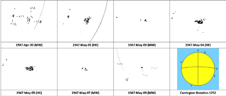
Figure 17. Passage of Greenwich group 14933, based on Mt Wilson (MW) and Hisako Koyama (HK) drawings.
