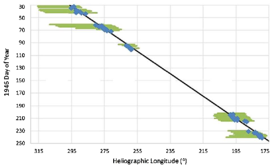
Figure 13. Longitude evolution of groups 14417 & 14585, including subsequent rotations.
