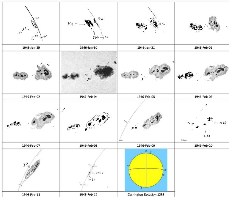
Figure 3. Passage of Greenwich group 14417 based on drawings, 18,19 and a photograph, 20 from Mt Wilson.
