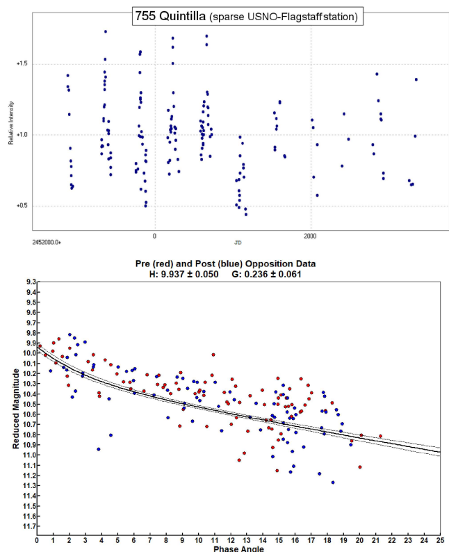
Figure 2: Top: sparse photometric data point distribution from (689) USNO Flagstaff station (relative intensity vs Julian Day). Bottom: phase curve obtained from sparse data (reduced magnitude vs phase angle).
