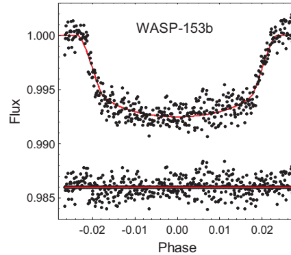
Fig. 2. The same as in Fig. 1 for WASP-153b.
