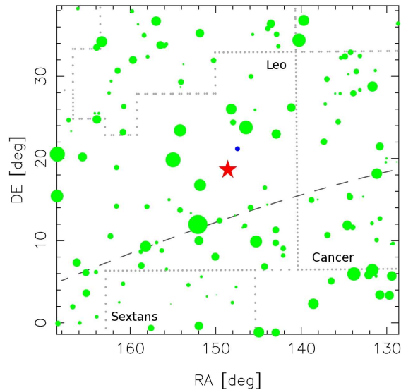
Figure 4. Southern \delta Leonids (#113, SDL), the third set of parameters for this shower contains the radiant coordinates RA=148.6 , DE=18.6 . Its ecliptic latitude is BE=5.5 degrees, what means that this radiant, marked by a star symbol, lies in the northern ecliptic hemisphere not the southern one.
