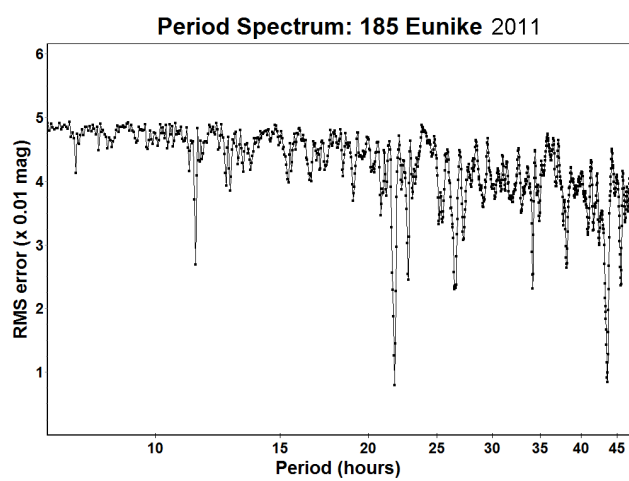
Figure 4. Period spectrum of year 2011 observations of 185 Eunike.
