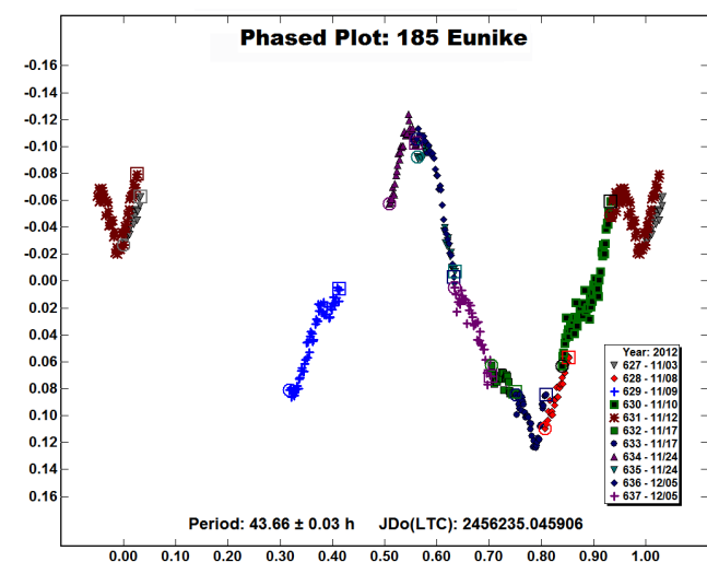
Figure 9. Year 2012 observations of 185 Eunike phased to the double period 43.66 hours.
