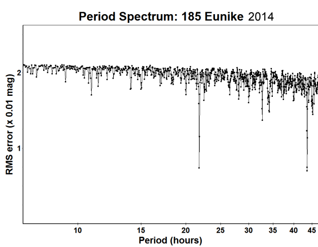
Figure 10. Period spectrum of year 2014 observations of 185 Eunike.
