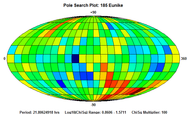
Figure 18. Pole Search Plot of \log(\text{ChiSq}) values, where dark blue identify lower \text{ChiSq} values and Dark red underlying the worst solutions.
