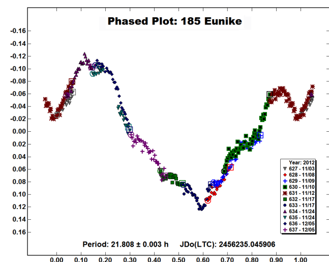
Figure 8. Year 2012 observations of 185 Eunike phased to a period 21.808 hours.
