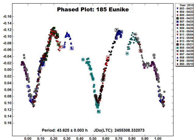
Figure 3. Year 2010 observations of 185 Eunike phased to the double period 43.625 hours.
