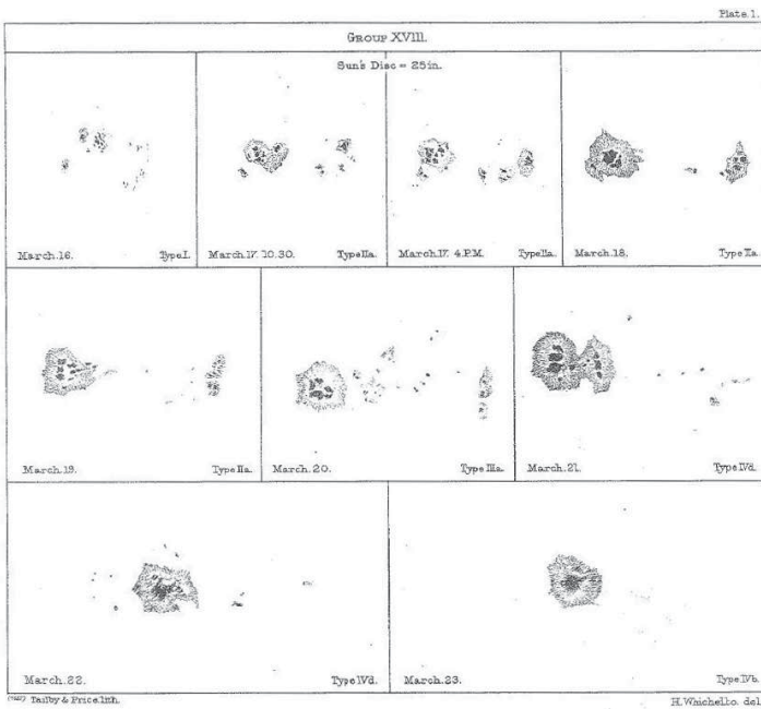
Figure 7. Evolution of a sunspot group during 1899 March. 61
