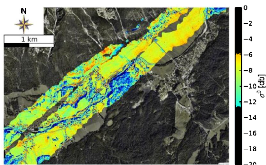
Figure 17. Geocoded SnowSAR backscatter image, Ku-band VV, three SAR swaths, Leutasch, 24 January 2013, on Google Earth image.
