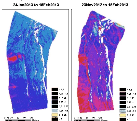
Figure 13. Change of snow depth (colour scale in metre) between individual campaigns for northern section of Rotmoos valley, derived from terrestrial laser scanner measurements.
