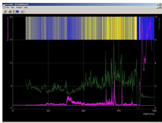
Figure 11. Display of SnowMicroPen profile near snow pit 2, Rotmoos, 8 January 2013. Purple: penetration resistance [N]. Green: texture index.
