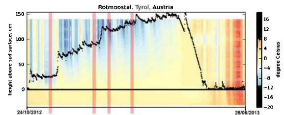
Figure 14. Snow height and temperature of snow and soil at the Rotmoos station, 24 October 2012 to 26 June 2013. Pink lines: field campaigns.
