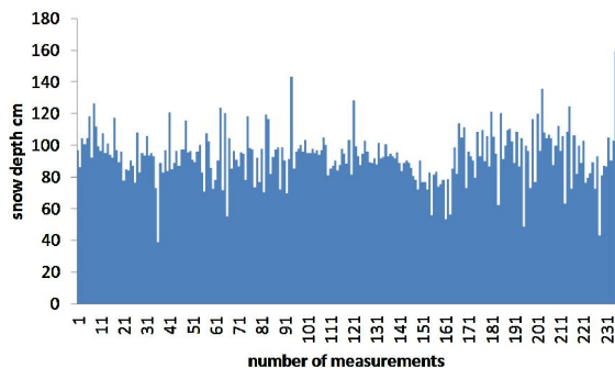
Figure 6. Snow depth of a transect along Rotmoos valley, 8 January 2013.
