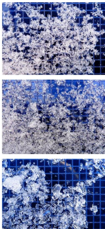
Figure 13. Photos of snow grains from three layers of snow pit 2, Rotmoos, 8 January 2013. 2 mm grid.
