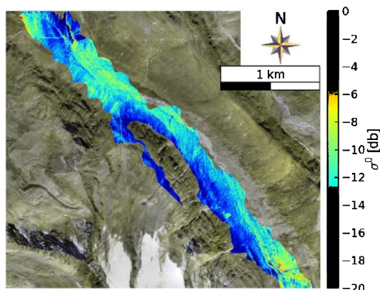
Figure 18. As Fig. 17, single swath, for Rotmoos, 24 January 2013.
