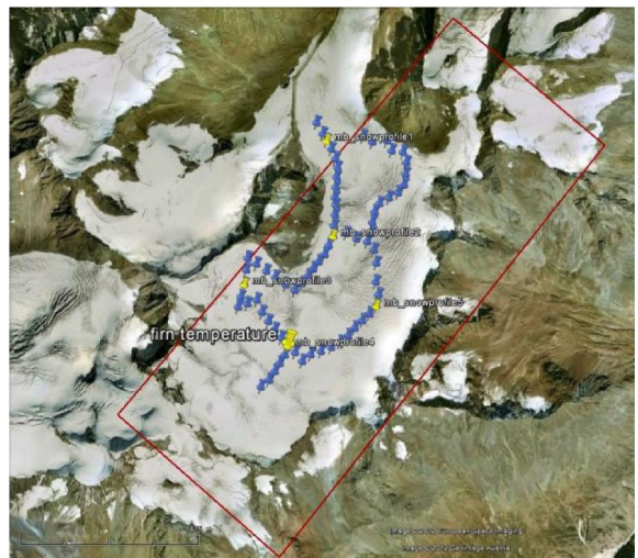
Figure 5. Test site Mittelbergferner on Google Earth image. The red box outlines the approximate area for SnowSAR acquisition. Blue pins: snow depth transects. Yellow pins: snow pits.
