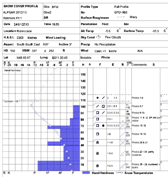
Figure 9. Example for protocol of snow pit measurements. Rotmoos, pit Nr.1, 24 January 2013.
