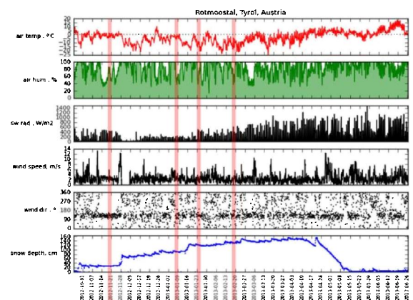
Figure 15. Meteorological parameters and snow height recorded at the Rotmoos station from 24 October 2012 to 26 June 2013.
