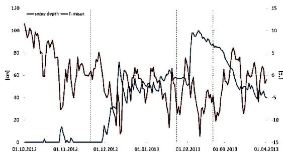
Figure 16. Snow depth and daily mean air temperature recorded at the station Leutasch-Kirchplatzl, 1 October 2012 to 1 April 2013. The dashed vertical lines indicate the dates of the three flight campaigns.
