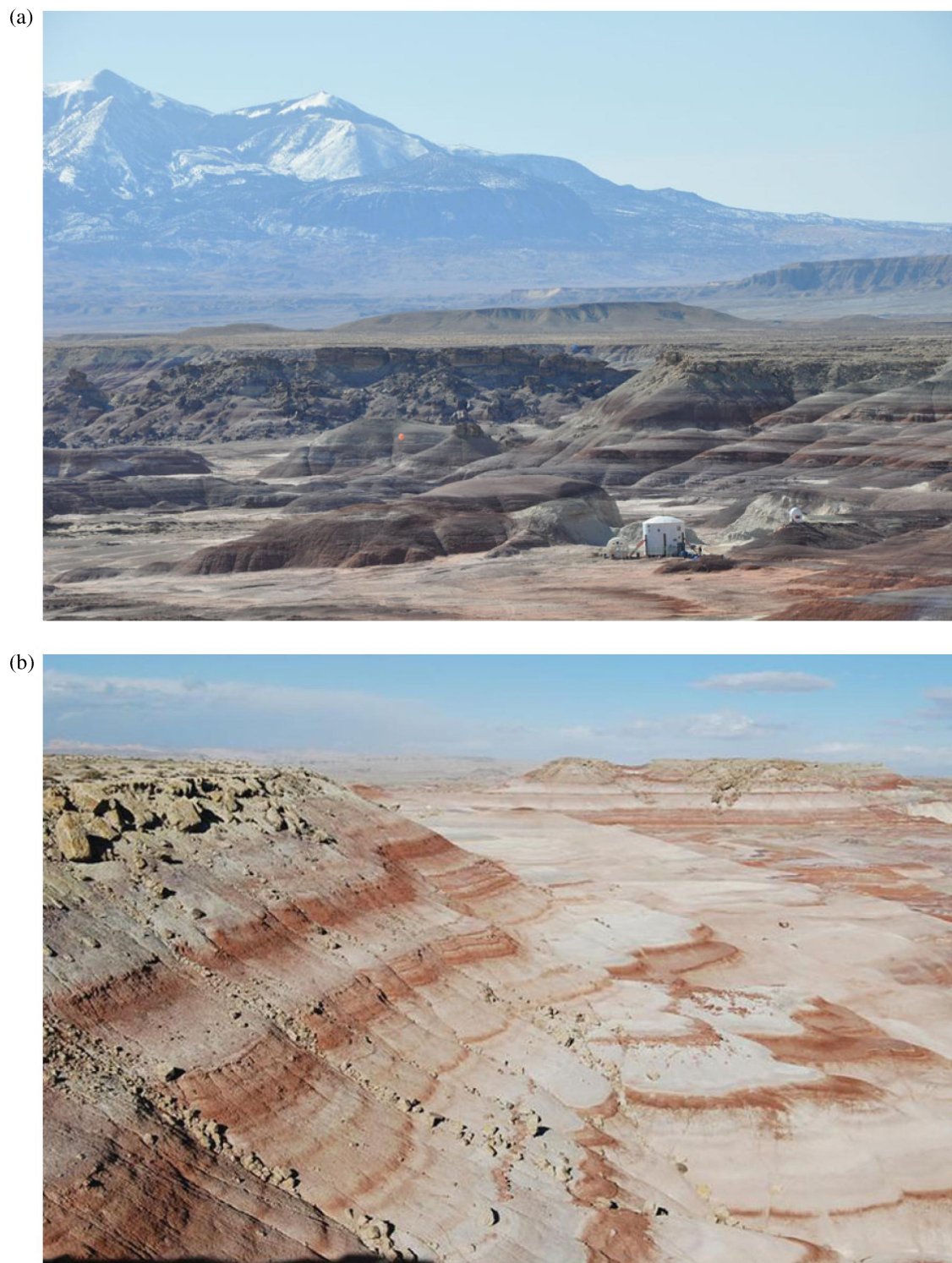
Fig. 2. (a) Southward view towards MDRS with Henry Mountains background. (b) Landscape and stratigraphy near MDRS station looking North, showing the resistant layer formed by sandstones of the Dakota sandstone formation at the top of the ridge and the shale slopes of the Brushy Basin member of the Morrison formation below.
