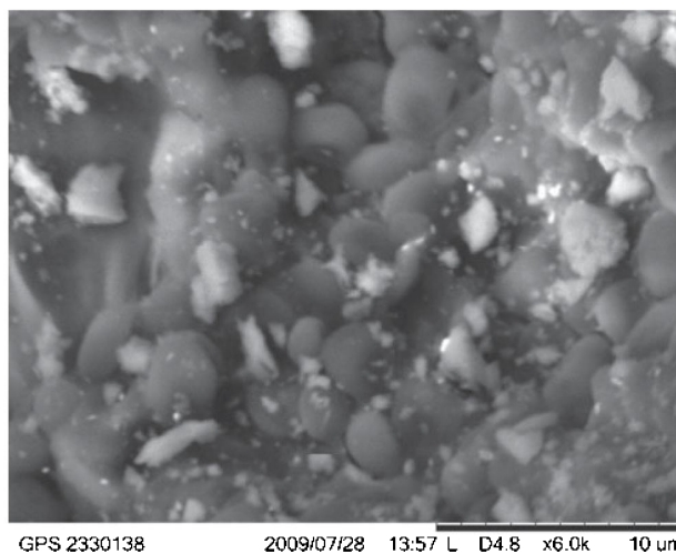
Fig. 19. SEM image of clump of coccoid cells, with abiotic particles suspended in a matrix possibly made of extracellular polymeric substance (EPS) from within an endolith.
