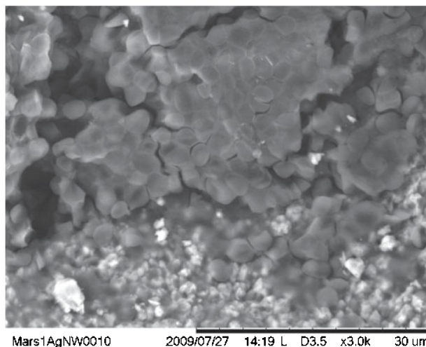
Fig. 18. SEM view of endolith coccoid cells (smooth round features) together with sandstone micron particles (jagged shapes).
