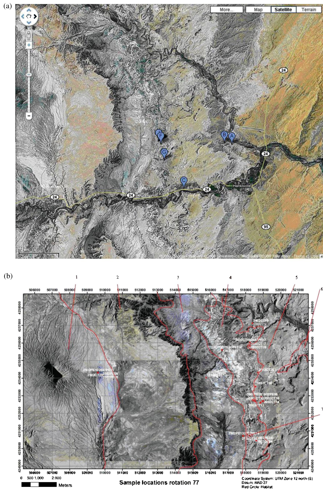
Fig. 1. (a) Google Earth satellite image showing the location of the MDRS station (near F) and sampling areas at Kissing Camel Ridge (near G). (b) Geology for the EuroGeoMars campaign, and positions of sampling areas (Wendt et al. 2009).
