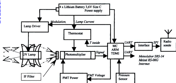
Figure 3. Block-diagram of FLASH-BM
