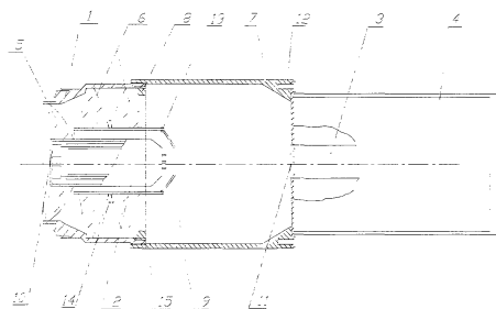
Fig. 1 Hygrometer design. 1 – kovar mounting, 2 – hydrogen lamp, 3 – photomultiplier, 4 – electronic unit, 5 – convex-concave lens, 6 – biconvex lenses, 7 – connecting tube, 8 – thread bushing, 9 – lamp housing, 10 – window-filter of the lamp, 11 – interference filter, 12, 13 – screw, 14 – teflon ring
