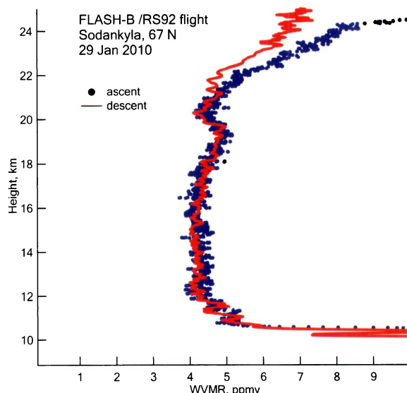
Figure 6. The results of balloon flight with new version of FLASH-BM.
