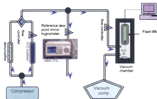
Figure 5. The scheme of calibration bench
