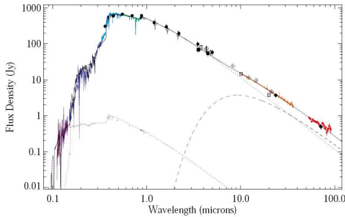
Figure 1: The ultraviolet-optical-infrared spectral energy distribution of epsilon Aurigae.
