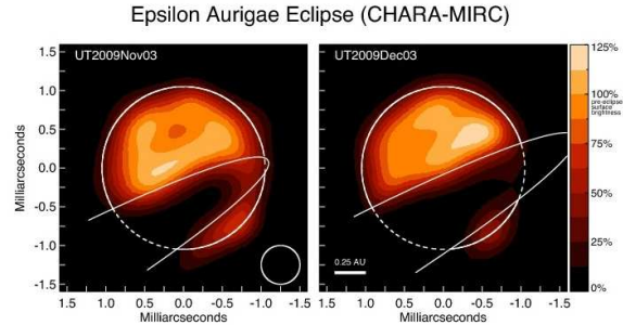
Figure 2: Ingress images of epsilon Aurigae, on the sub-milli arcsecond spatial scale, during ingress 2009 November and December.
