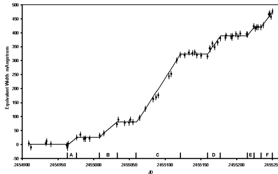
Figure 3: Variation of the excess equivalent width of neutral potassium in epsilon Aurigae during ingress.
