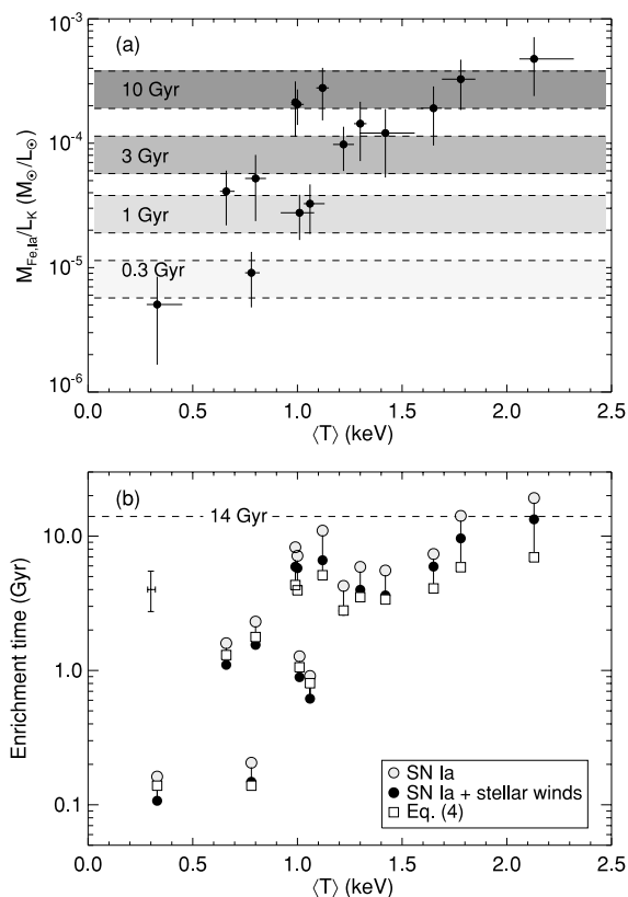
Figure 12. (a) Mass of Fe produced by SN Ia within 0.1r_{500} , normalized to the K-band luminosity of the central group galaxy. Shaded regions outline the errors on the typical time-scales required for SN Ia to produce the observed M_{\text{Fe}}/L_K ratios, assuming a constant SN Ia rate with redshift. (b) The corresponding enrichment times, including also the effect of stellar mass loss in the BGG, and that of assuming an SN Ia rate evolving with redshift according to equation (4). Lines connect the time-scales for each group as computed under these different assumptions. A typical error bar (dominated by uncertainties in the local SN Ia rate) is shown at T = 0.3 keV. Dashed line marks an enrichment time-scale of 14 Gyr.
