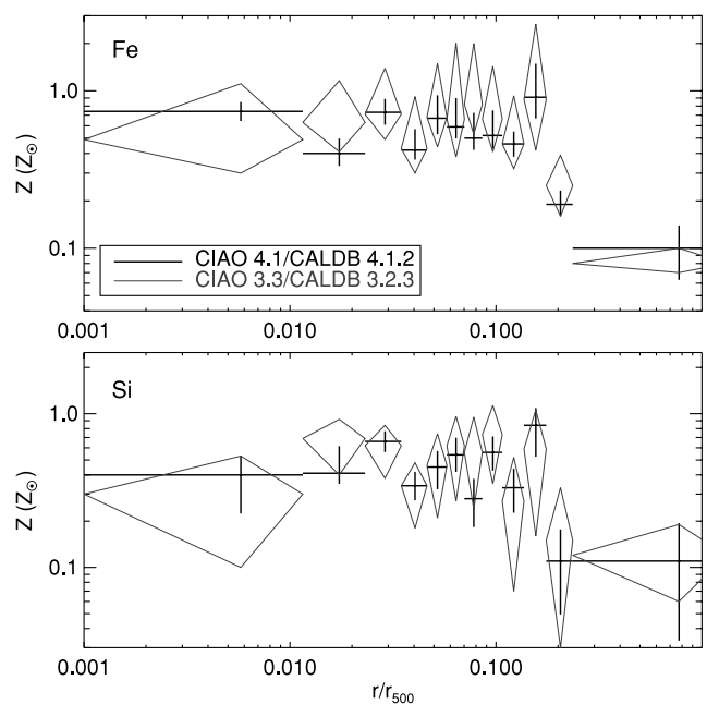
Figure 4. Comparison of (top) Fe and (bottom) Si profiles derived for NGC 4325 using the most recent Chandra calibration data (black crosses) and those of our original analysis in Paper I (grey diamonds).
