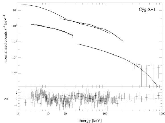
Figure 1. Best fit to the observation of 2004 November 20/21 (obs2) using the eqpair model. There are slight indications for a hard tail, but this could also be due to instrumental uncertainties.
