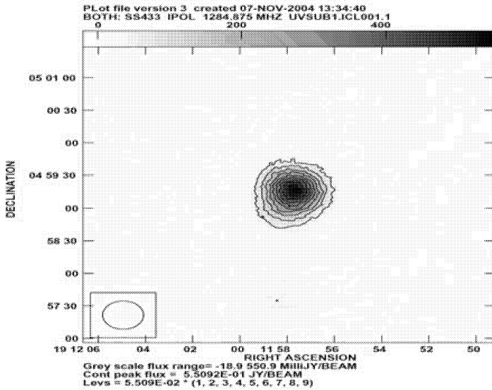
Figure 2. (a) Radio and (b) IR images of SS 433. This radio image taken on 2002 October 1 is at 1.28 GHz. The peak flux is \sim 0.55 \text{ Jy beam}^{-1} . The size of the beam is given in the lower left. The contours are at intervals of \sim 0.055 \text{ Jy} . The IR image taken on 2002 September 27 is in the J band. The standard stars (1 and 2) referred in the text are also shown. The magnitudes are given as well.
