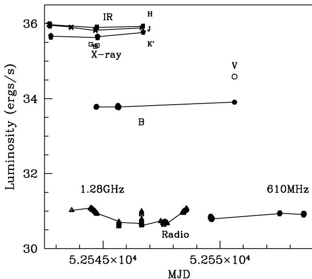
Figure 3. Multi-wavelength observation of SS 433 at 1.28 GHz (triangles) band and at 610 MHz (filled hexagons) in radio, at J (crosses), H (filled circles), K' (filled pentagons) bands in IR, B (filled circles) and V (open circle) bands in optical, and 3–25 keV (open squares) in X-ray during the campaign. There seems to be a lag of minimum intensity region in the radio (MJD 52545.5 to MJD 52547.5) with respect to the infrared minimum region ( \sim MJD 52544–52545) by about 2 d.
