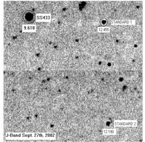
Figure 2. (a) Radio and (b) IR images of SS 433. This radio image taken on 2002 October 1 is at 1.28 GHz. The peak flux is \sim 0.55 \text{ Jy beam}^{-1} . The size of the beam is given in the lower left. The contours are at intervals of \sim 0.055 \text{ Jy} . The IR image taken on 2002 September 27 is in the J band. The standard stars (1 and 2) referred in the text are also shown. The magnitudes are given as well.
