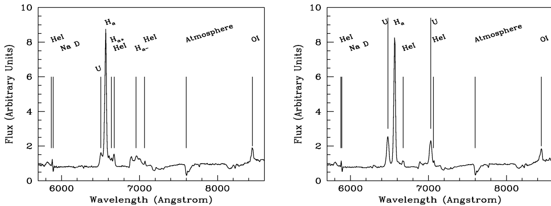
Figure 7. The calibrated, continuum-subtracted, optical spectrum of SS 433 on 2002 September (a) 27 and (b) 28. In (a) the H_\alpha line, blue- and red-shifted H_\alpha lines (denoted by H_{\alpha+} and H_{\alpha-} respectively), HeI lines, OI line, atmospheric and sodium absorption lines are identified. The Doppler-shifted H_\alpha lines are exactly where they are expected from kinematic model of Abell & Margon (1979) within the instrumental resolution of 5 \text{ \AA} . In (b) we also see two bright lines, marked by 'U' at 7029.07 and 6481.09 \text{\AA} respectively.
