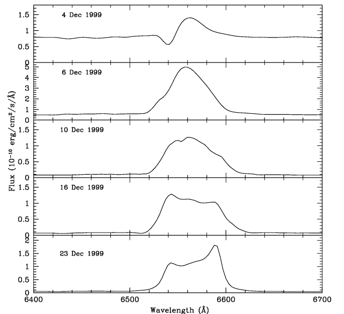
Figure 3. Evolution of the H \alpha line showing the transition from an optically thick wind to a polar blob–equatorial ring geometry.
