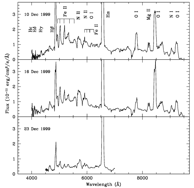
Figure 2. Spectra of V1494 Aql in the early decline phase. The gradual hardening of the spectrum is reflected in the weakening of Fe II lines and the sustained strength of lines of higher ionization.
