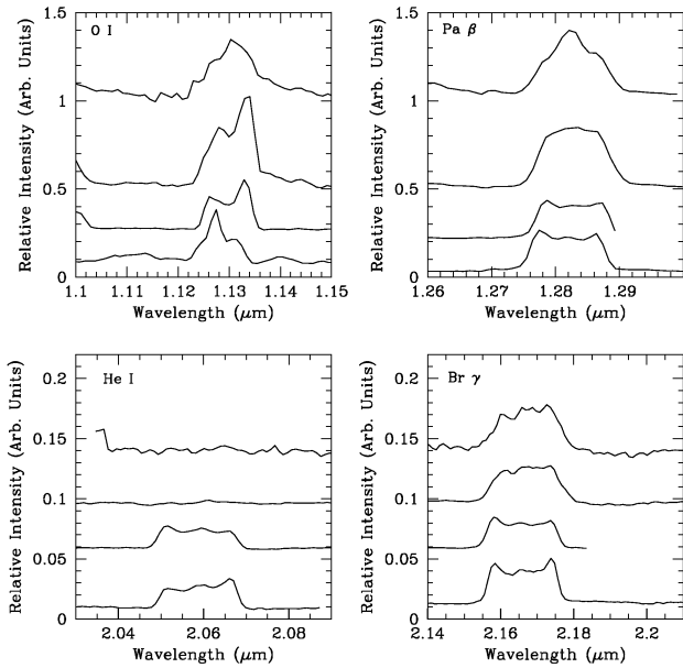
Figure 10. Evolution of some near-infrared emission line profiles seen in the early (1999 December – top) to the later (2000 March – bottom) spectra. The spectra have been shifted or scaled for illustrative purposes.
