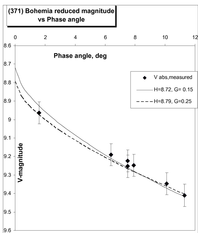
Figure 4. Reduced magnitude vs. Phase angle.
