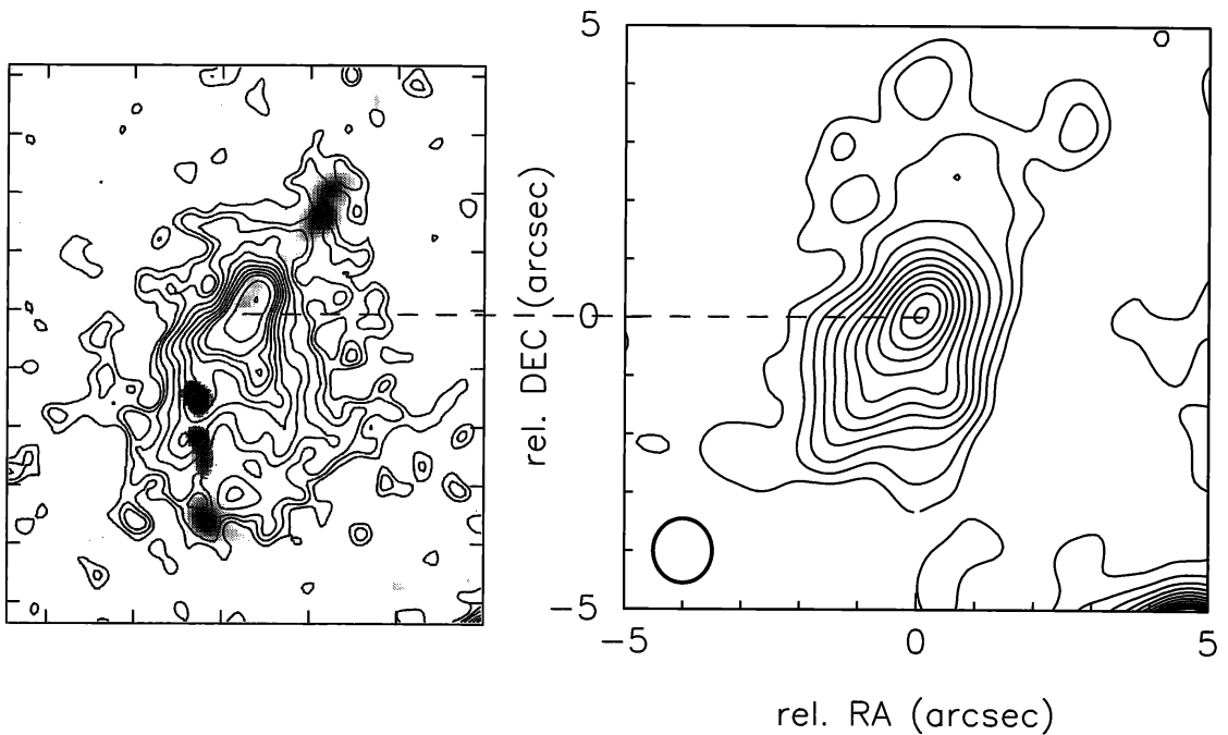
Figure 1. Our V-band image of 1243+036 (right), which includes the redshifted Ly \alpha emission, compared with the narrow-band Ly \alpha image (contours), overlaid on the radio 8GHz image (gray scale), of vO96 (left) at a same scale. The V-band image is smoothed by Gaussian convolution to enhance the weak emission at outer parts of the nebula; the effective seeing (after the smoothing) is 1."1 FWHM, as shown by a circle at the lower left corner.
