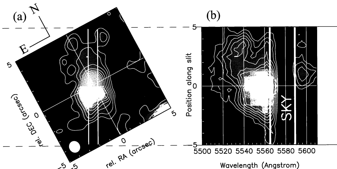
Figure 2. Our two-dimensional Ly \alpha spectrogram (right) is shown as well as the slit position overlaid on our V-band image (left). The V-band image is rotated so that the slit position, indicated by two lines at the nebula center, is seen vertically. The spectrogram is smoothed by 4 by 4 pixel running average to enhance the outer weak emission. After the smoothing, the effective resolution is 1.''2 in space which is almost comparable to that of the smoothed imaging data, and the velocity resolution is 600 \text{ km s}^{-1} . The wavelength region where no information is available due to residual strong [O I] sky emission at 5577\text{\AA} is masked out.
