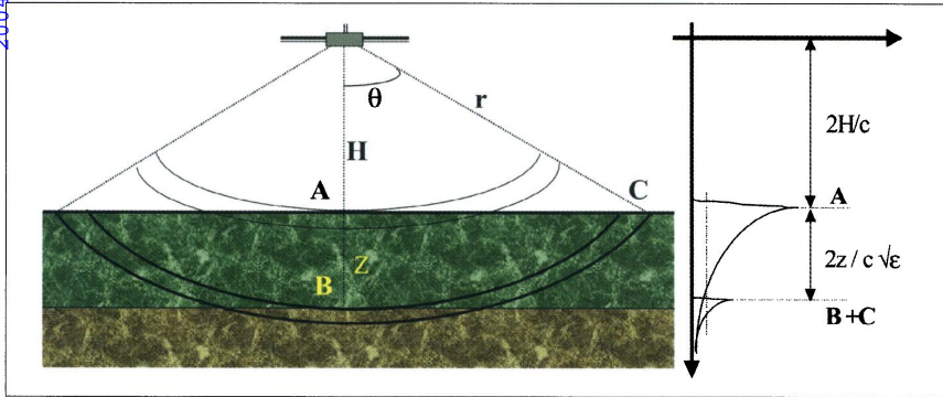
Fig. 4. MARSIS observation geometry and principle of operation.
