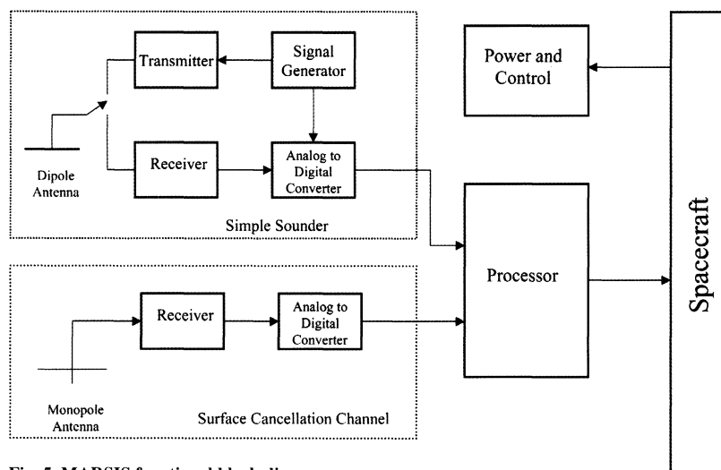
Fig. 5. MARSIS functional block diagram.
