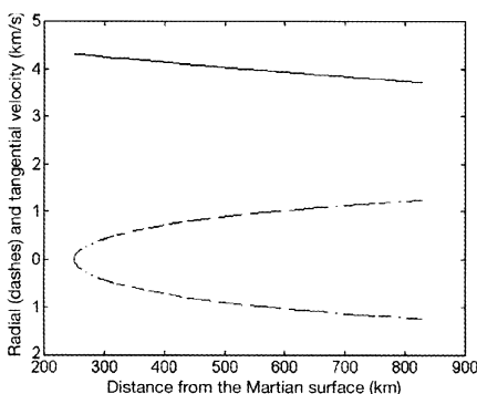
Fig. 3. Radial and tangential spacecraft velocity.
