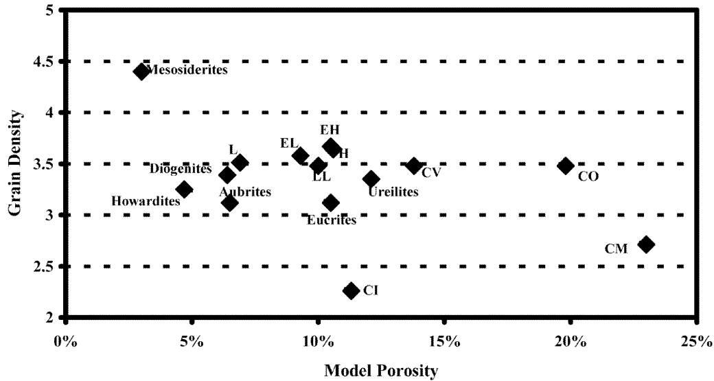
Fig. 1. Grain density versus model porosity for the major meteorite groups. This plot emphasizes how anomalous the CI and CM carbonaceous chondrites are relative to the vast majority of stony meteorites. Most stony meteorites are clustered between 3.0 and 3.7 g/cm 3 , while CI and CM meteorites are much less dense. The mesosiderites are also outliers because of their high iron content.
