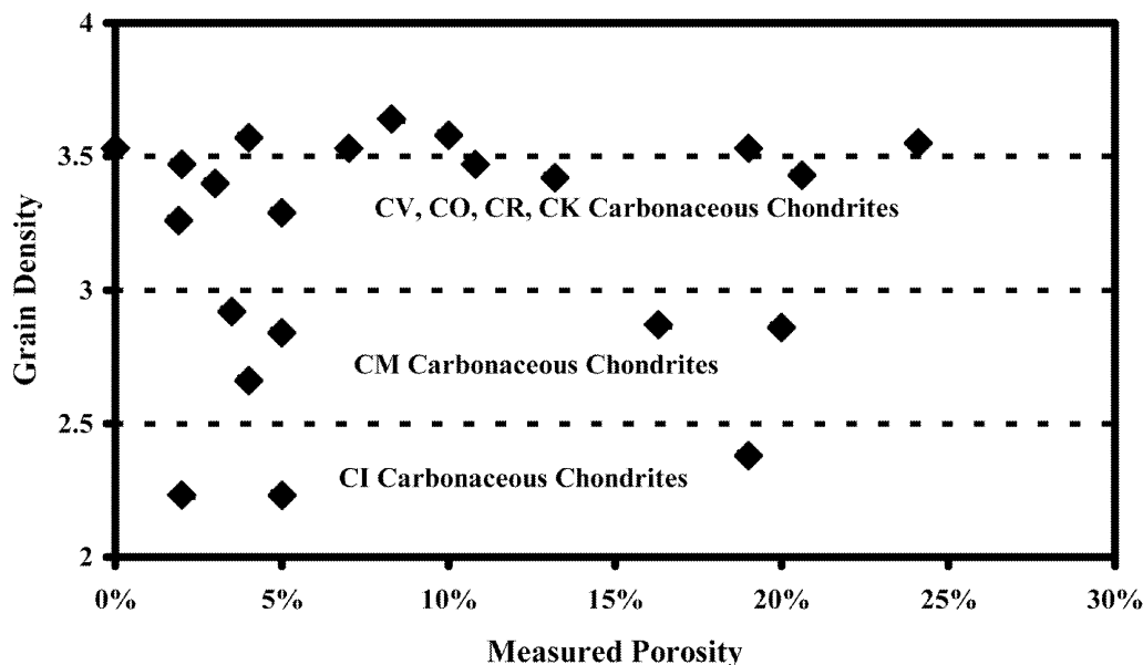
Fig. 2. Carbonaceous chondrite porosities and grain densities. Note that the vast majority of carbonaceous chondrites have grain densities clustering around 3.5 \text{ g/cm}^3 , similar to other stony meteorites such as ordinary chondrites. The exceptions are the CMs and CIs, which are rich in low-density hydrated silicates.
