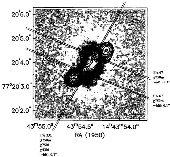
Fig. 3. Same as Fig. 1 but for 3C303.1. NOTE: THIS FIGURE IS AVAILABLE IN COLOR IN THE ELECTRONIC VERSION OF THIS ARTICLE, OBTAINABLE FROM http://www.astroscu.unam.mx/~rmaa/ .
