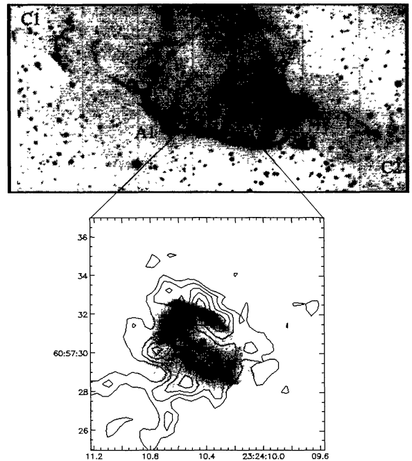
Fig. 2. A deep H\alpha mosaic of KjPn 8. The whole nebula is 14' \times 4' in extent. Inset: a contour map of excited 2.122 \mu\text{m H}_2 is shown overlaid on the [S \text{ II}] HST image of the core of KjPn 8. The \text{H}_2 , ionized and a larger CO disk, not shown here, all share morphology and orientation and their plane is perpendicular to the A_1 – A_2 high-velocity bipolar outflows.
