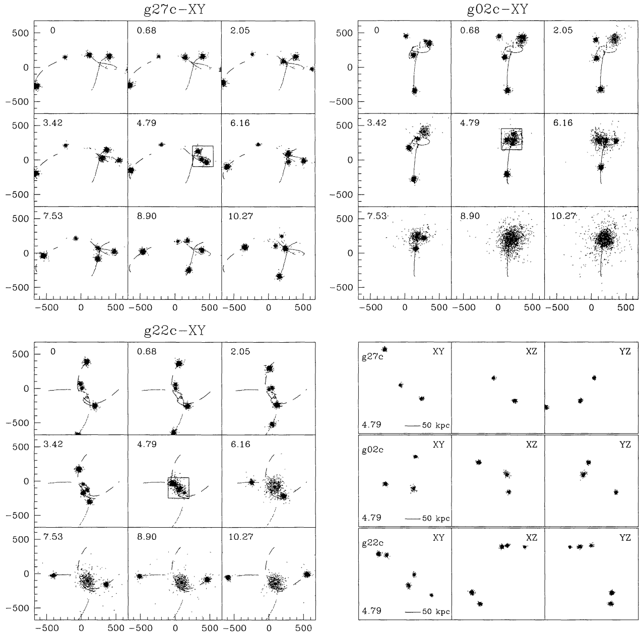
Fig. 1. This figure shows the XY-projection in kpc for the collapsing groups g27c (upper-left), g02c (upper-right) and g22c (bottom-left). The numbers in each frame indicate the time elapsed since turnaround in Gyr. Lines refer to the trajectories followed by each galaxy inside its corresponding group. Also, small boxes of width 300 kpc are shown at time 4.79 Gyr for each group. These boxes have been amplified and show just 'luminous' particles at the bottom-right of this figure which corresponds to the XY, XZ and YZ-projections.
