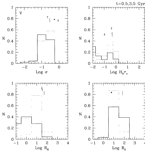
Fig. 7. Same as in Fig. 5, but for small groups with virial initial conditions.
