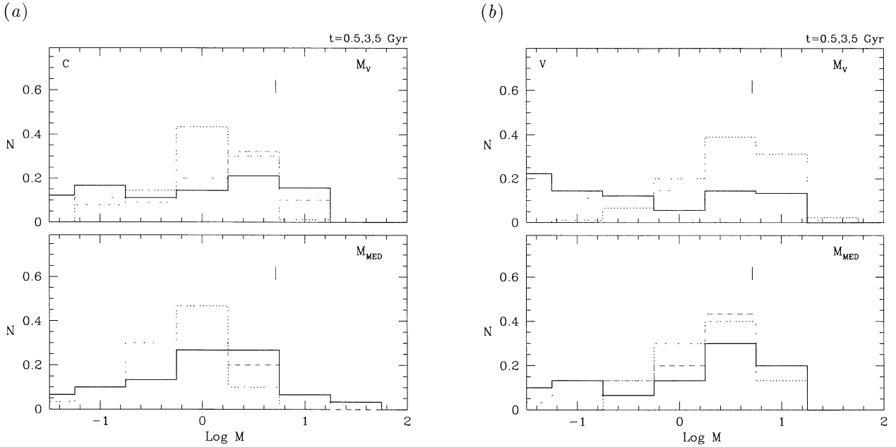
Fig. 9. Histograms of the behavior of the VME (upper panels) and MME (lower panels), for (a) cold and (b) virial small groups. The bar (|) indicates the true mass of the groups in N -body units. Dotted lines show the distribution at t = 0.5 Gyr, short-dashed lines at 3 Gyr, and solid at 5 Gyr.
