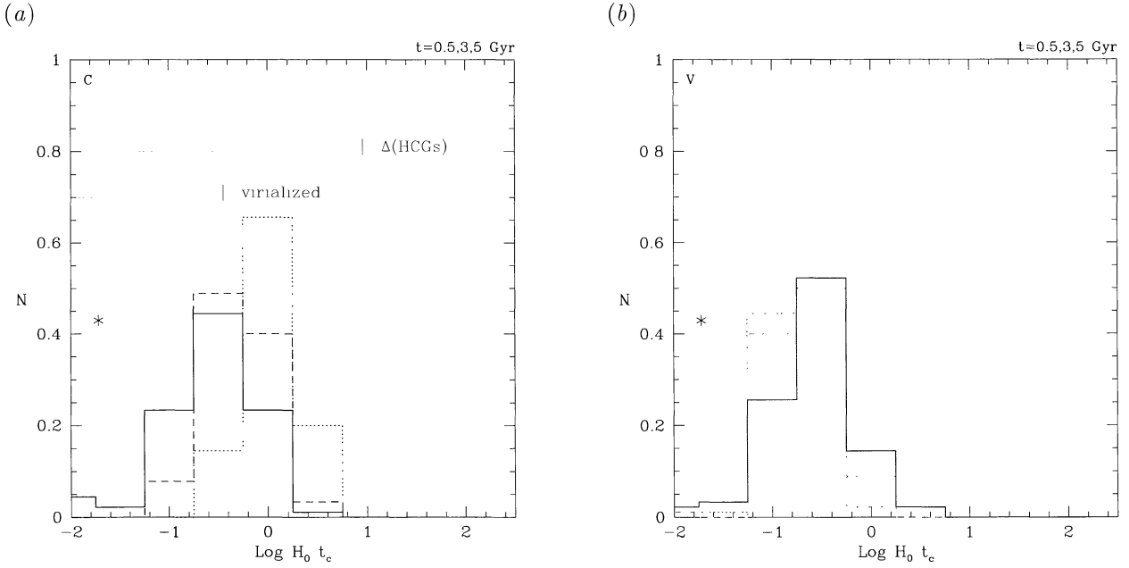
Fig. 6. Evolution of the distribution of the crossing-time t_c = R_S/(\sqrt{3}\sigma) . Line styles are the same as in Fig. 5. The interval of crossing-times for HCG and that assumed to be satisfied by virialized groups, according to the criterion of Gott & Turner (1977), are indicated. (a) Results for collapsing groups. (b) Results for virialized groups. Note that both kinds of initial conditions lead to ranges in crossing-time within the observed values.
