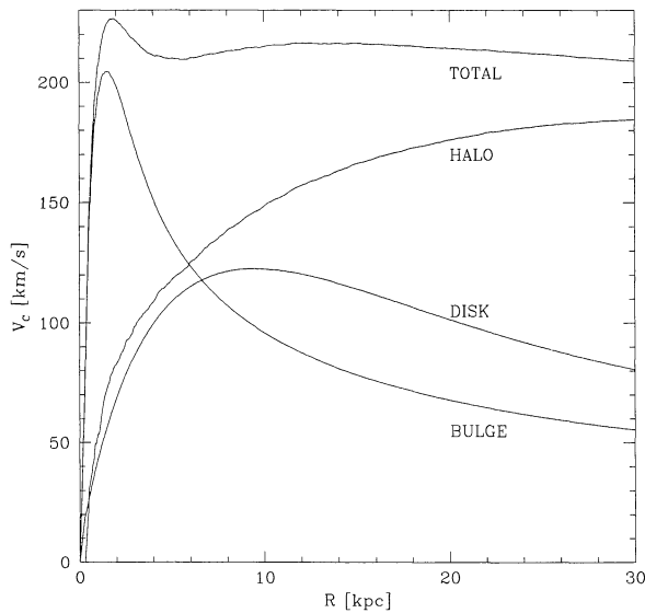
Fig. 11. Rotation curve for the spiral galaxy model.
