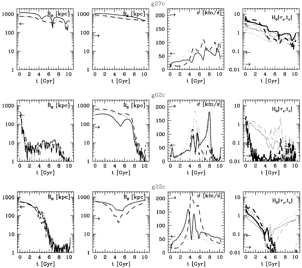
Fig. 4. Kinematical parameters as a function of time for collapsing groups g27c , g02c , and g22c . Astronomical units are used. The left-arrow ( \leftarrow ) indicates the median of the 5-galaxy MK groups, while the right-arrow ( \rightarrow ), HCG. The different lines indicate the line-of-sight used to compute the quantities: along X-axis (solid), along Y-axis (dotted), and along Z-axis (broken). For the dimensionless crossing times, thicker lines for H_0\tau_c than for H_0t_c have been used.
