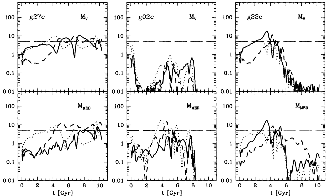
Fig. 8. Time behavior of the two mass estimators considered in § 5 for our collapsing groups g27c , g02c , and g22c . The upper panels show the virial mass, while the lower the median mass. The horizontal broken line corresponds to the total mass of the groups; N -body units are used for the mass, but physical units for the time. The different types of line denote different lines-of-sight, as in Fig. 4.
