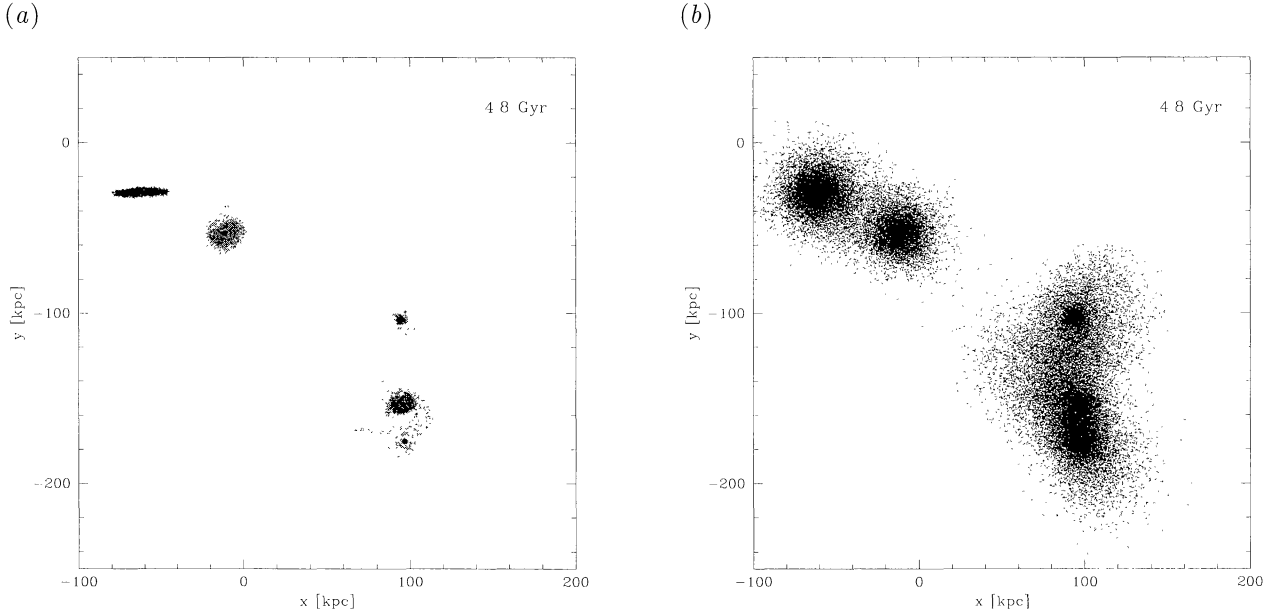
Fig. 12. XY-projection at time 4.8 Gyr of our more realistic model. Luminous particles are shown in (a) and the dark component is indicated in (b). Note that a common dark envelope for the three galaxies close to merging is already present, while the other two in the upper-left will not merge for \gtrsim 5 Gyr from the present epoch. Compare with our previous model g22c of Fig. 1.
