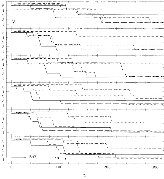
Fig. 3. As in Fig. 2, but for initially virialised groups. In this case, the arrow corresponds to the dynamical time of the group.
