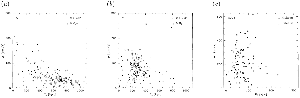
Fig. 10. R_s - \sigma diagram for (a) collapsing, (b) virialized, and (c) Hickson's groups. Hickson's compact groups appear to resemble systems that have suffered a gravitational collapse out of a more diffuse system.
