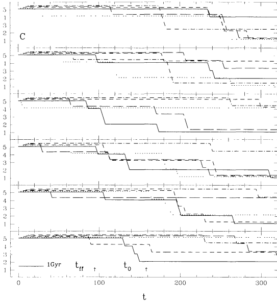
Fig. 2. Number of individual galaxies versus time (merging history) for simulations with cold initial conditions. The free-fall time-scale (Mamon 1990) t_{\text{ff}} = \pi \sqrt{R_{\text{rmax}}^3 / (32GM_G)} and the present epoch t_0 ( \sim 5 Gyr from ‘turnaround’) are indicated by arrows. The merging tracks have been displaced vertically and in time for better appreciation. The displacement in time corresponds to 0, 3, 6, 9, and 12 time units. A scale corresponding to 1 Gyr is indicated.
