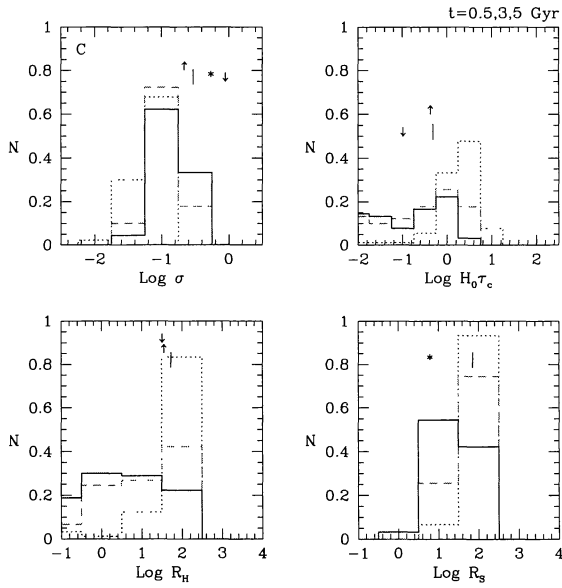
Fig. 5. Collapsing groups: Histograms of the velocity dispersion, mean harmonic radius, dimensionless crossing time ( H_0\tau_c ), and mean separation at different times. The different symbols denote the median for HCG (*), NCfA (|), and MK groups (†). Hickson Compact Groups Associations' values (Ramella et al. 1994) are also indicated (↓) for completeness. Different line styles correspond to different times of evolution: 0.5 Gyr (dotted), 3.0 Gyr (short-dashed), and 5 Gyr (solid).
