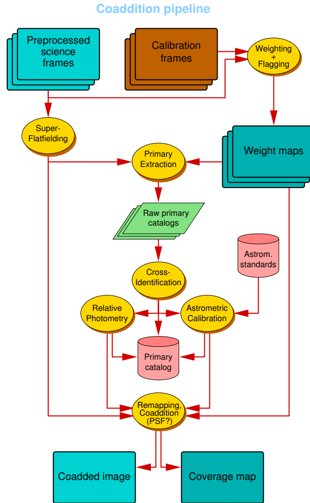
Figure 3. Global overview of the SWarp package.
