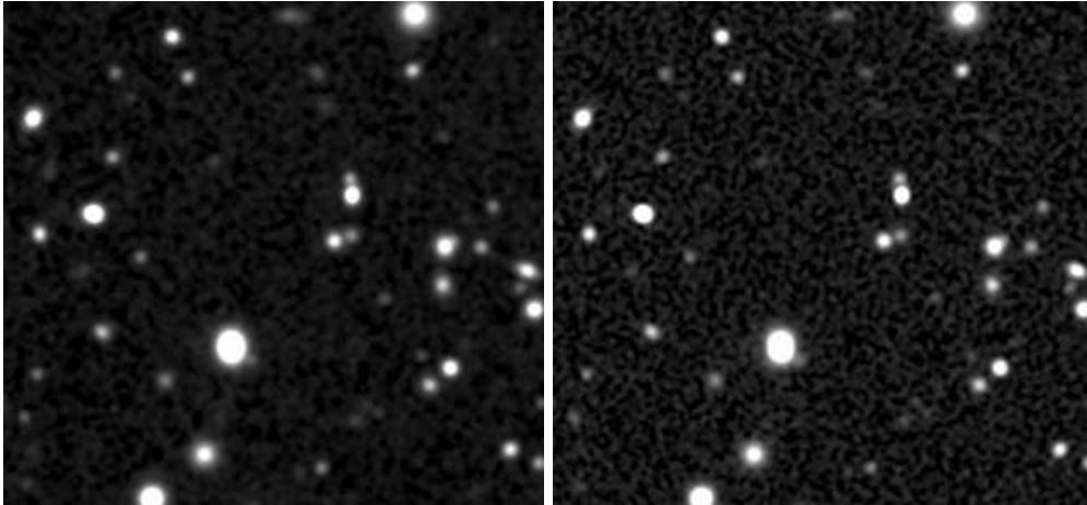
Figure 6. Test of PSF homogenization on simulated images. Left: MEGACAM image with an original seeing of 0.6'' , degraded to 0.75'' ; right: MEGACAM image of the same field (same exposure time) with an original seeing of 0.9'' , sharpened to 0.75'' .
