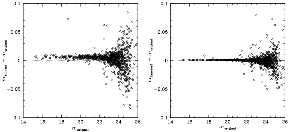
Figure 5. Effects of resampling on flux measurements. Left: bilinear interpolation; right: Lanczos3 interpolation. In both cases, a simulated deep sky image with 0.7'' seeing, containing stars and white background noise, was rotated by 20 degrees and then rotated back to match the original image. Fluxes were measured in a fixed 2'' aperture. The dispersions reflect the differences between measurements on the original and resampled images. These dispersions are much smaller than what one would observe by comparing the measurements on the resampled images with the theoretical (noise-free) fluxes of the simulation. Note the significant dispersion in magnitude for the bilinear case, a consequence of the stronger smoothing induced by bilinear interpolation.
