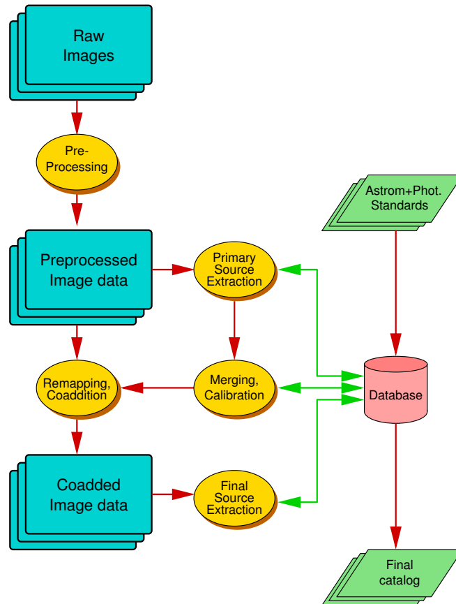
Figure 2. Global overview of the TERAPIX pipeline.
