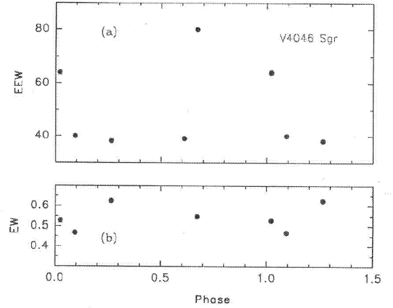
Fig. 2.— Plots of (a) H\alpha EEW and (b) Li I EW.
