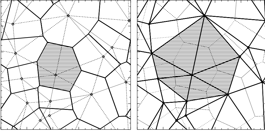
Fig. 1. A set of 20 points with their Voronoi (left frame: solid lines) and Delaunay (right frame: solid lines) tessellations. Left frame: the shaded region indicates the Voronoi cell corresponding to the point located just below the center. Right frame: the shaded region is the “contiguous Voronoi cell” of the same point as in the lefthand frame.
