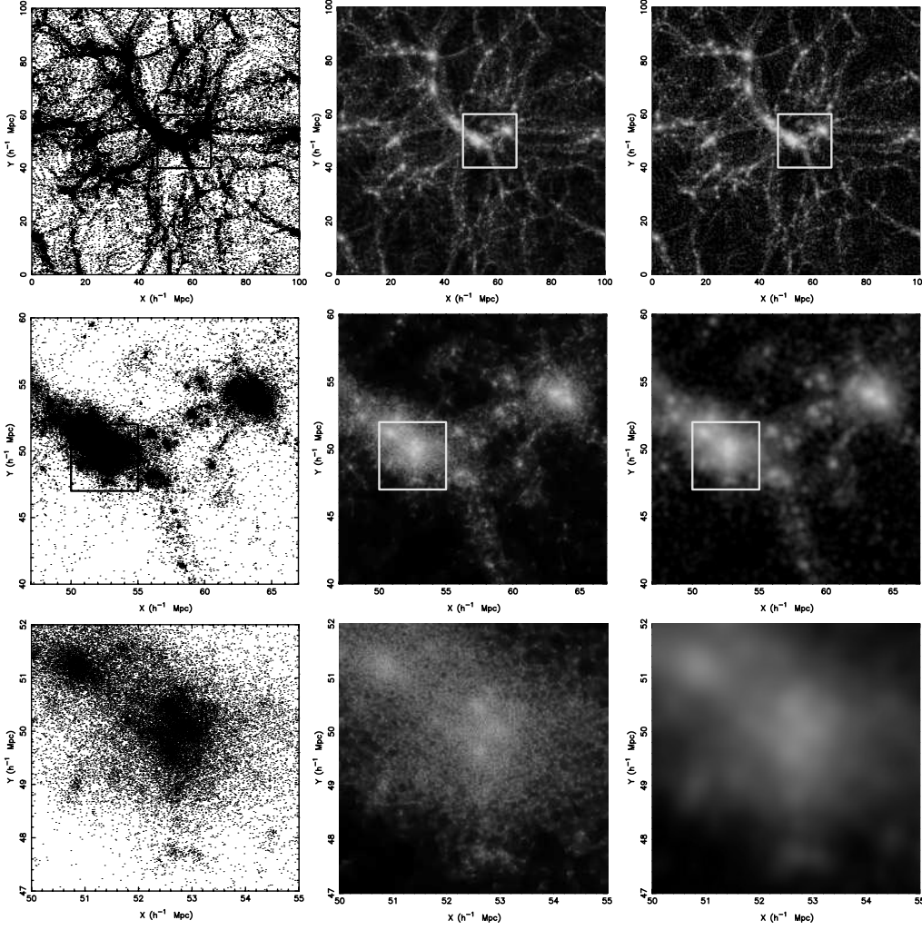
Fig. 2. A 9-frame mosaic comparing the performance of the Delaunay density estimating technique with a conventional grid-based TSC method in analyzing a cosmological N-body simulation. Left column: the particle distribution in a 10h^{-1}\text{Mpc} wide central slice through the simulation box. Central column: the corresponding Delaunay density field reconstruction. Right column: the TSC rendered density field reconstruction. The colour scale of the density fields is logarithmic, ranging from \delta\rho/\rho = 0 - 2400 .
