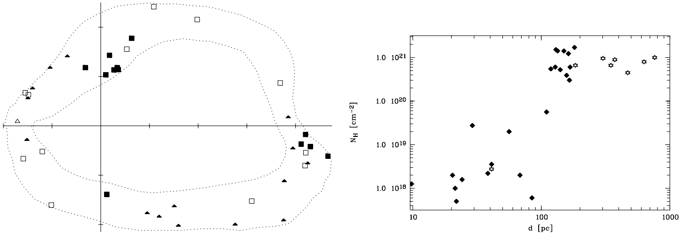
Fig. 8. Left: Positions of stars projected onto the annular X-ray shadow cast by the interaction ring. Filled symbols (triangles: d < 80 pc, squares: d > 80 pc) denote stars with HIPPARCOS distances while open symbols represent stars without these new distances. The galactic plane ( b = 0^\circ ) as well as the center ( l = 0^\circ ) are indicated with tics at each 20^\circ . Right: H I column densities towards stars projected onto the interaction ring, again filled symbols stand for stars with HIPPARCOS distances and empty symbols for stars without. Clearly, N_{\text{H}} rises to \sim 7 \times 10^{20} \text{ cm}^{-2} at around 100 pc. Absorption data taken from Fruscione et al. (1994).
