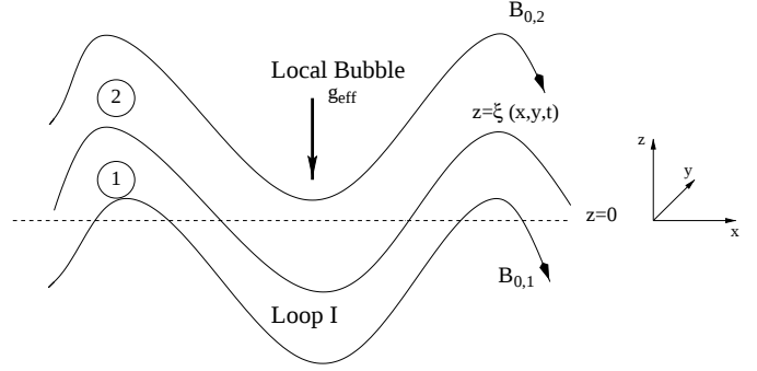
Fig. 3. Sketch of the tangential boundary between Loop I and the Local Bubble. The magnetic field is different, but constant on either side. The gravitational pull due to the weight of the fluid is a function of \xi(x, y, t) .
