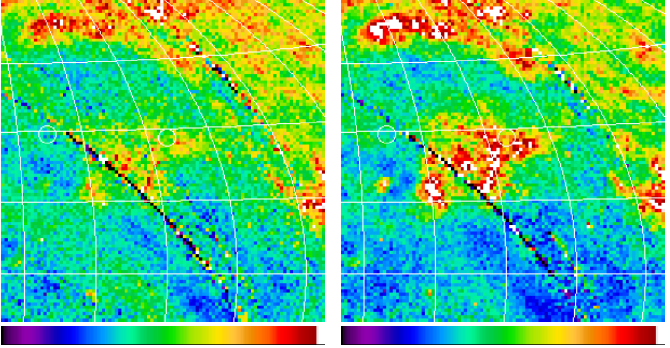
Fig. 6. ROSAT PSPC survey X-ray intensity maps of the central part of the Loop I region in the R1 (left, PSPC channels 8 – 19, \sim 0.08 – 0.28 keV, dynamic range 0 – 450 \times 10^{-6} counts s^{-1} arcmin ^{-2} ) and R2 (right, channels 20–41, \sim 0.15 – 0.28 keV, 0 – 650 \times 10^{-6} counts s^{-1} arcmin ^{-2} ) band in galactic coordinates in Aitoff-Hammer projection. The pixel size is 40 arcmin. Coordinate lines are in steps of 15^\circ starting at l = 345^\circ (left) and b = 0^\circ (bottom), the two regions with \chi^2 -contour analysis (Fig. 7) are indicated by circles (A1 right, A2 left). Errors in the band rates (R1, R2) in the selected regions (A1, A2) are less than 4% at the 1\sigma level while the difference between A1 (bright) and A2 (dark) exceeds 34%.
