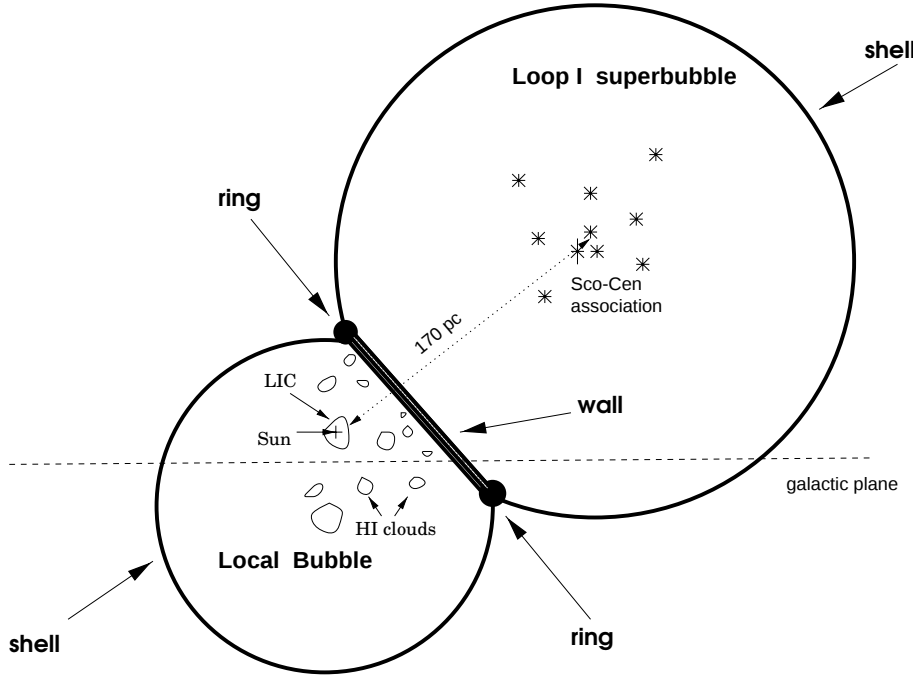
Fig. 1. Schematic representation (not drawn to scale) of the interaction between the Local Bubble and the neighbouring Loop I superbubble (longitudinal cut perpendicular to the galactic plane). The dark slab represents the dense, compressed interaction zone (“wall”), bounded by the “ring”, as seen in absorption in the ROSAT images. Also shown are H I cloudlets that seem to be associated with the wall and have systematic velocities pointing towards us.
