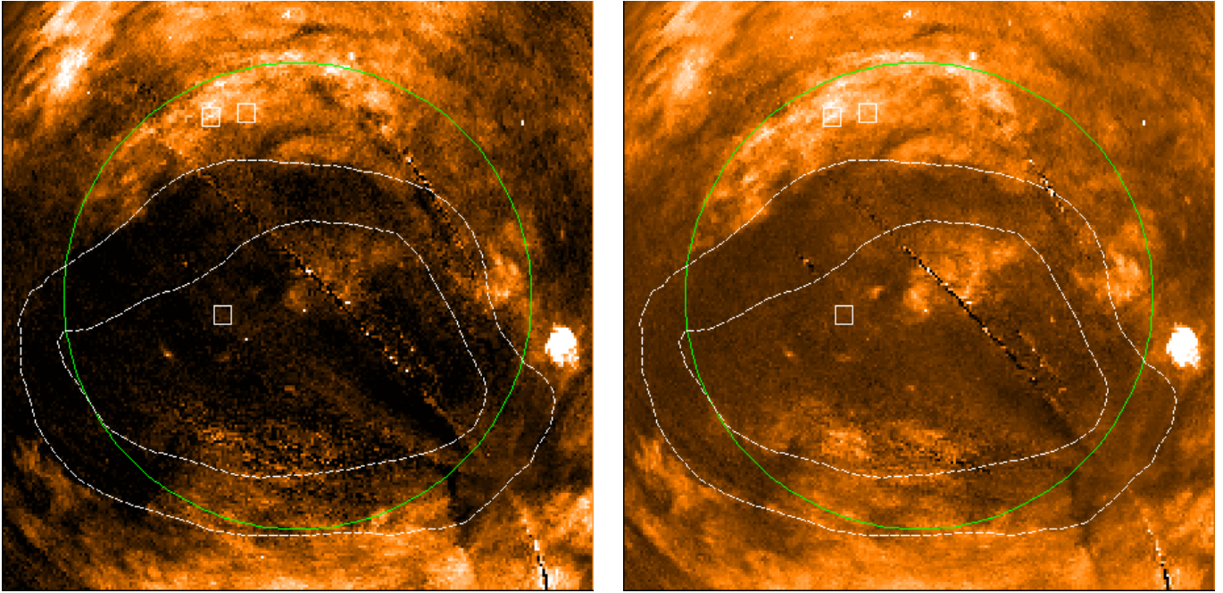
Fig. 5. ROSAT PSPC maps of the Loop I region in the R1 (left) and R2 (right) band centered on the centre of the radio continuum (RC) Loop I, (l, b, r) = (330^\circ, +17.5^\circ, 58^\circ) . Dashed white lines mark the contours of the H I ring formed by the interaction of Loop I with the LB as described in Egger & Aschenbach (1995). For details see text.
