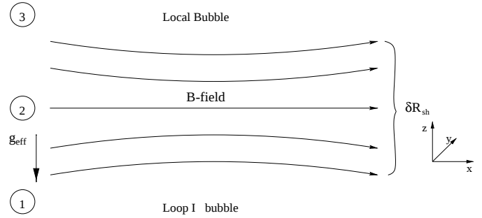
Fig. 2. Sketch of the compressed interaction zone of thickness \delta R_{\text{sh}} between Loop I and the Local Bubble. If the magnetic lines of force are antiparallel, magnetic reconnection will produce a neutral current sheet in which resistive dissipation occurs, thus weakening the field in the wall. The curvature of the shell boundaries is overemphasized.
