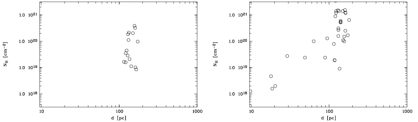
Fig. 9. H I column densities of stars in the direction of the ring and towards the wall with b > 5^\circ as a function of HIPPARCOS distances. Left: N_{\text{H}} derived from Na I absorption measurements. Right: N_{\text{H}} derived from all other methods (e.g., Ly \alpha , Mg II, EUV). The rise in column density to N_{\text{H}} \sim 10^{20} \text{ cm}^{-2} occurs at a distance of \gtrsim 60 pc, thus indicating the existence of a wall. H I column densities derived from Na I appear to be lower, the sampling in distance is not as complete as in the right panel. Absorption data taken from Fruscione et al. (1994).
