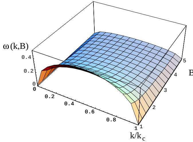
Fig. 4. The growth rate \omega(k, |\mathbf{B}|) in arbitrary units as a function of wave vector k (in units of k_c ) and magnetic field strength |\mathbf{B}| = \sqrt{B_{0,1}^2 + B_{0,2}^2} in units of \mu\text{G} .
