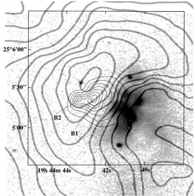
Fig. 1. CO emission (thick grey lines) and radio continuum emission (thin black lines) superimposed on an \text{H}\alpha frame of the Sh2-88B region (B1950 coordinates). The CO J = 2-1 emission is from White & Fridlund (1992); in this map the antenna temperature is integrated over a velocity channel of 1 \text{ km s}^{-1} centered at 22 \text{ km s}^{-1} – the velocity of the ionized gas at the head of the cometary B1 structure. The radio continuum emission at 8.3 GHz is from Garay et al. (1998b). The \text{H}\alpha frame was obtained at the Observatoire de Haute Provence with the 120-cm telescope. North is up and east is left. The size of the field is 2'.1 \times 1'.8 .
