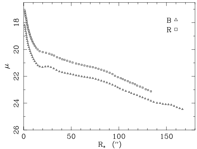
Fig. 3. Averaged radial profiles in each individual photometric pass band as a function of the equivalent radius of each isophotal level.
