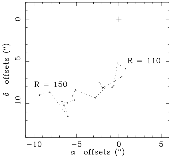
Fig. 6. Position of the centers of the R isophotes from radius = 110'' to 150'' , showing a drift with increasing radius of \sim 11'' to the SE.
