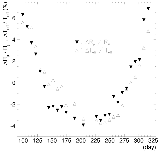
Figure 4: Temperature and rate variations superimposed, with \Delta R_\mu / \langle R_\mu \rangle scaled by the value of \alpha_T determined in this analysis.
