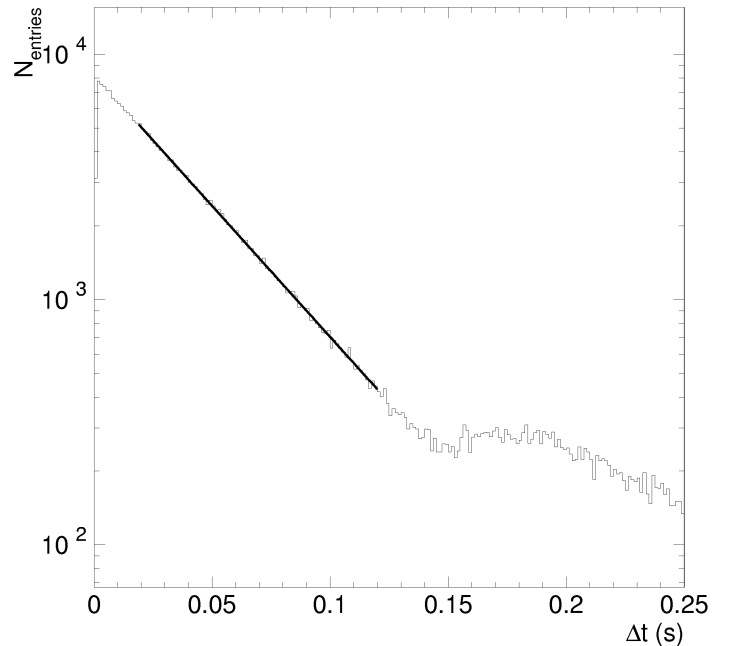
Figure 1: Distribution of the time between triggered events \Delta t . This figure shows the fit for data taken during day 120.
