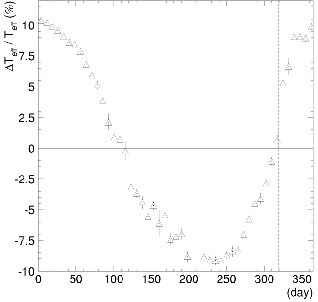
Figure 3: The relative variation of the effective temperature around its mean \Delta T_{eff} / \langle T_{eff} \rangle as a function of day number for the full year 1997. The dotted lines show the 225-days period when our muon data was taken.
