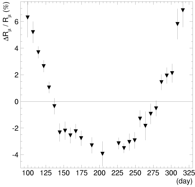
Figure 2: The measured relative variation of the trigger rate around its mean \Delta R_\mu / \langle R_\mu \rangle as a function of day number, for the 225 days used. The data is sorted in bins of 7.5 days.
