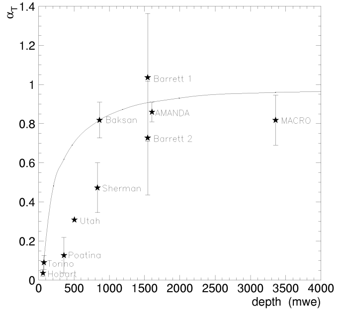
Figure 5: Measurements of \alpha_T by detectors at different depths, with the expected curve and with the AMANDA value added. Taken from (Ambrosio et al., 1997).
