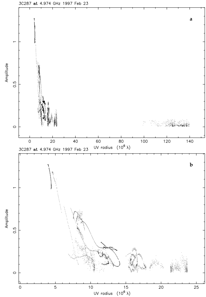
Fig. 2a and b. Correlated flux density (Jy) versus projected baseline length: a all data including baselines to Shanghai telescope, b the western EVN, 0–25 M \lambda u–v range
