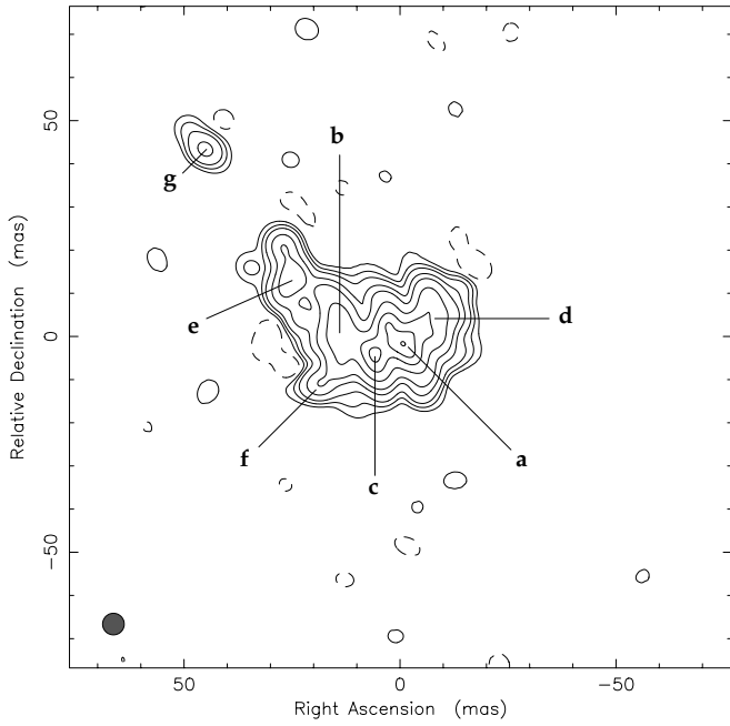
Fig. 1. Natural weighted image of 3C287 at 5 GHz. Contour levels are -0.4, 0.4, 1, 2, 5, 10, 25, 50, 75, 99 % of the 183 mJy peak flux density. The restoring beam is 5 mas
