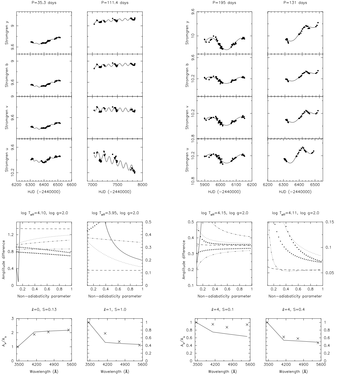
Fig. 7. Top four panels: multicolour data for the four passbands of the Strömgren system of R 127 (two left panels) for the period 1 and 2 (see Table 4) and for S Dor (two right panels) for the period 1 and 2. The dots are the observations while the full lines are fits with the pulsation periods listed in Table 4 and given on top of each panel. Middle panels: The amplitude differences (in magnitudes) as a function of the non-adiabaticity parameter (see text for an explanation) for the most likely degrees of the pulsations. Different symbols denote different degrees: full line: \ell = 0 , dashed line: \ell = 1 , dotted line: \ell = 2 , dashed-dotted line: \ell = 3 , dashed-dot-dot-dot line: \ell = 4 , \star : \ell = 5 , \times : \ell = 6 . Lower panels: the observed amplitude ratios A_x/A_u for x = u, v, b, y (crosses) are compared with those of the best theoretical model (connected by the full line) for the four filters of the Strömgren system
