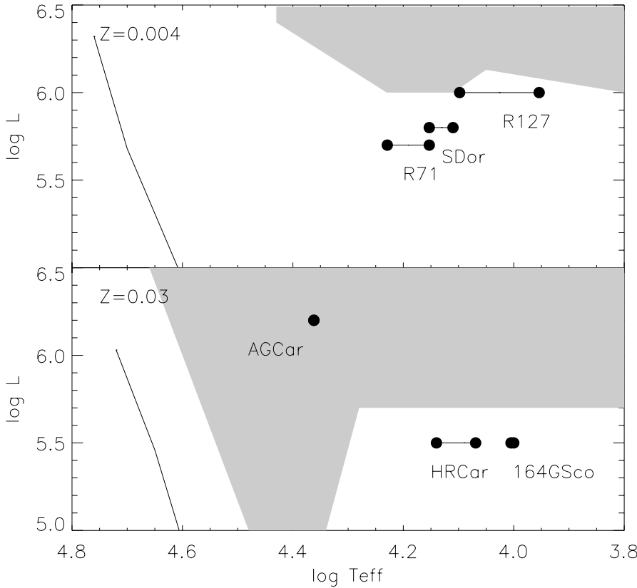
Fig. 5. The location of the strange-mode instabilities in the HR-diagram (shaded area) for Z = 0.004 and Z = 0.03 (from Kiriakidis et al. 1993). The location of our LMC program stars at the time of the observed variability are compared with the predictions of Z = 0.004 and the Galactic stars are compared with Z = 0.03 . The left full line indicates the location of the main sequence.
