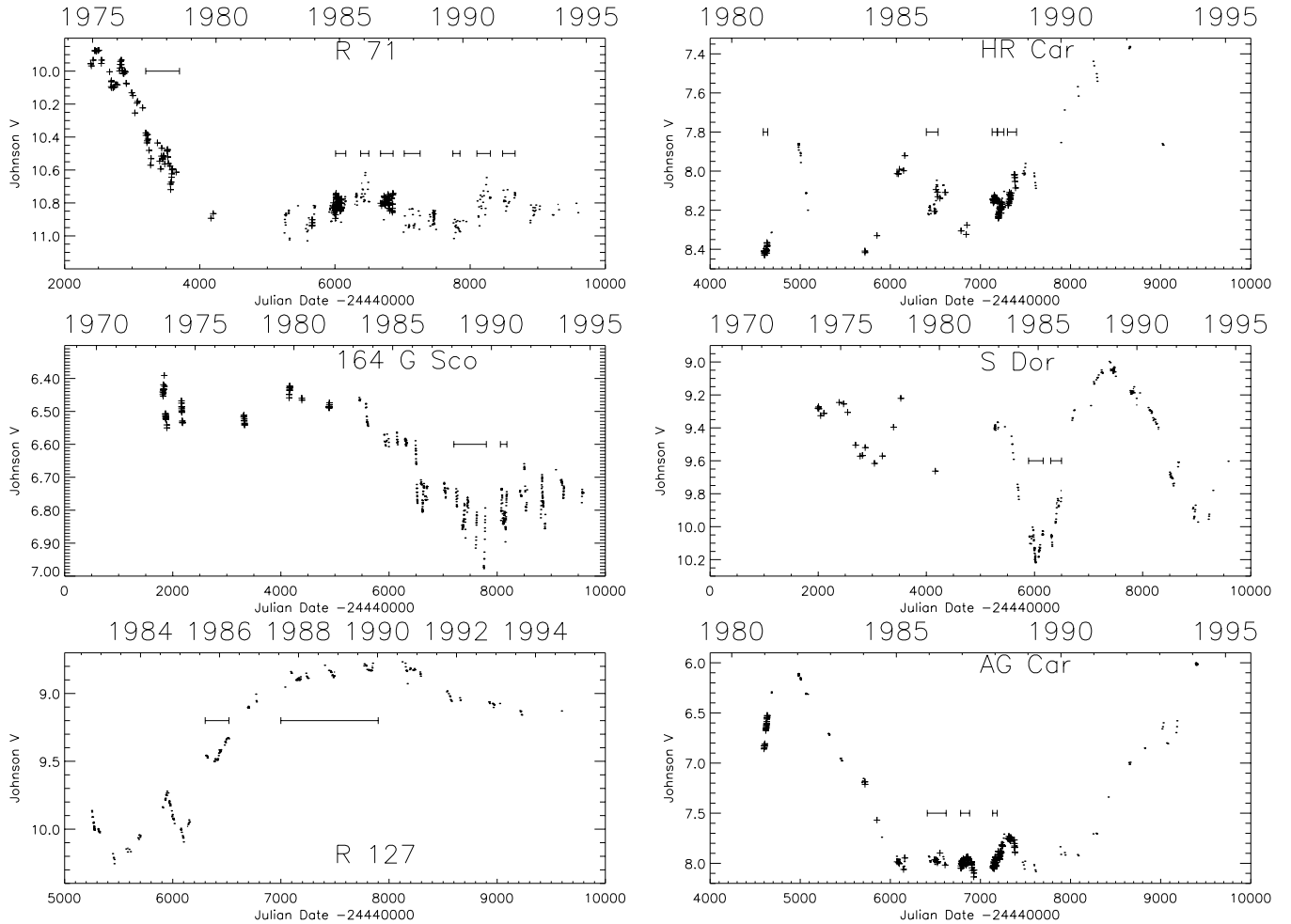
Fig. 1. The light curves of the program stars over periods of about 12 to 25 years (data collected by Spoon et al. 1994). Different symbols refer to data from different photometric systems (see Spoon et al.). The horizontal bars indicate the time intervals in which we found periodicity of the microvariations.
