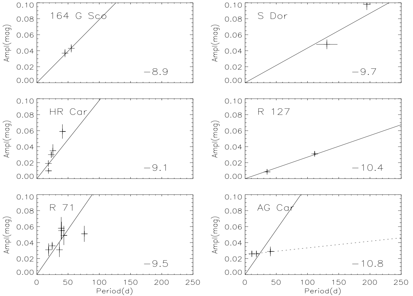
Fig. 4. The amplitude versus period of the microvariations. The stars are arranged in order of increasing luminosity, with the value of M_{\text{bol}} indicated in the lower right corner. The lines are linear fits going through zero with a slope given in Table 6. For AG Car we also show the slope of the relation that does not go through the zero point.
