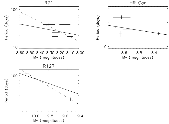
Fig. 3. The values of \log P versus M_V for three stars. The dashed lines show the weighted least square fits. The full lines show fits with a fixed slope of 0.505, which is predicted for adiabatic radial pulsations for constant Q and M_{\text{bol}} .
