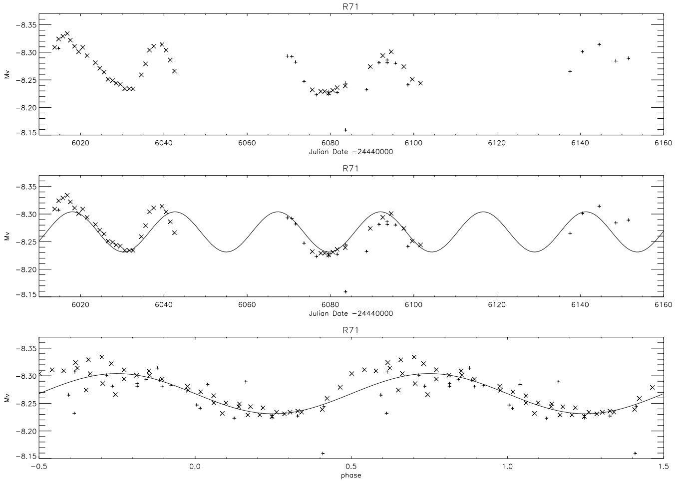
Fig. 2. a The photometric data of R 71 between Nov 1984 and April 1985; b The data with a sine wave of the calculated frequency; c The data folded with a sine wave. The lightcurve is given by two different symbols because the measurements were done with two different instruments (Spoon et al., 1994)
