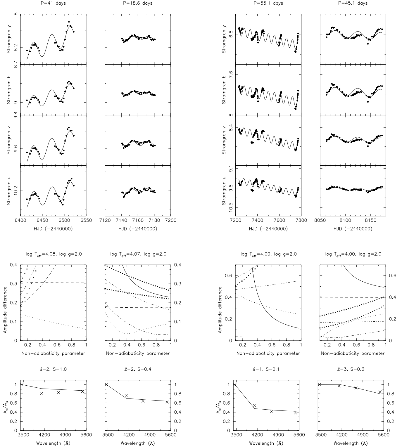
Fig. 6. Top four panels: multicolour data for the four passbands of the Strömgren system of HR Car (two left panels) for the period 2 and 3 (see Table 4) and for 164 G Sco (two right panels) for the period 1 and 2. The dots are the observations while the full lines are fits with the pulsation periods listed in Table 4 and given on top of each panel. Middle panels: the amplitude differences (in magnitudes) as a function of the non-adiabaticity parameter (see text for an explanation) for the most likely degrees of the pulsations. Different symbols denote different degrees: full line: \ell = 0 , dashed line: \ell = 1 , dotted line: \ell = 2 , dashed-dotted line: \ell = 3 , dashed-dot-dot-dot line: \ell = 4 , \star : \ell = 5 , \times : \ell = 6 . Lower panels: the observed amplitude ratios A_x/A_u for x = u, v, b, y (crosses) are compared with those of the best theoretical model (connected by the full line) for the four filters of the Strömgren system
