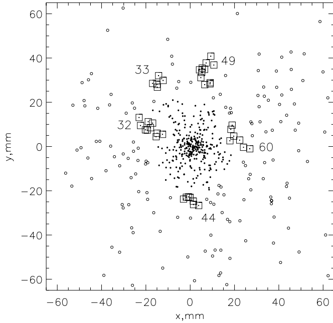
Fig. 1. Distribution of stars in the M 67 cluster in the rectangular coordinate system (x,y) centered at \alpha = 8^h47^m7 , \delta = +12^\circ . Squares show stars belonging to stellar groups with more than 5 members. Open circles – stars belonging to the corona. Numbers of groups are indicated
