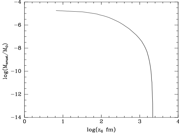
Fig. 3. \log(M_{crust}) vs. \log(z_G) . The mass of the strange core ( M_{core} ) is 1.4 M_\odot , its radius ( R_{core} ) is 1.097 \times 10^6 cm, which is evaluated by solving TOV equation numerically
