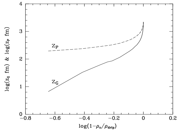
Fig. 2. \log(z_G) (the full line) and \log(z_p) (the dashed line) vs. \log(1 - \rho_c / \rho_{drip}) . Notice that abscissa of 0 corresponds to \rho_c \rightarrow 0 while abscissa of -\infty corresponds to \rho_c \rightarrow \rho_{drip} .
