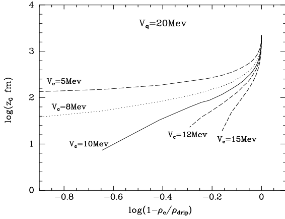
Fig. 4. \log(z_G) vs. \log(1 - \rho_c/\rho_{drip}) for V_q = 20 Mev. This figure shows the influence of the uncertainty of parameter V_c on z_G . The five lines from top to bottom correspond to V_c = 5, 8, 10, 12, 15 Mev respectively
