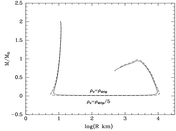
Fig. 6. Mass ( M ) vs. radius ( R ) for strange star–strange dwarf sequence. The full line is plotted with \rho_c equals \rho_{drip} and the dashed line with \rho_c = 8.332 \times 10^{10} \text{ g cm}^{-3}
