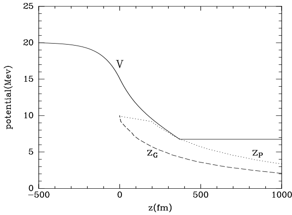
Fig. 1. Electrostatic potential ( V ) vs. height ( z ) near the surface of a strange star (full line). Density at the base ( \rho_c ) is chosen as 1.32 \times 10^{11} g cm -3 . The dashed line shows V_c vs. gap width ( z_G ) and the dotted line shows V_c vs. z_p .
