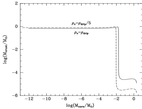
Fig. 7. Crust mass ( \log(M_{\text{crust}}) ) vs. the mass of strange core ( \log(M_{\text{core}}) ) for strange star–strange dwarf sequence. The full line is plotted with \rho_c = \rho_{\text{drip}} and the dashed line with \rho_c = \rho_{\text{drip}}/5 = 8.332 \times 10^9 \text{ g cm}^{-3}
