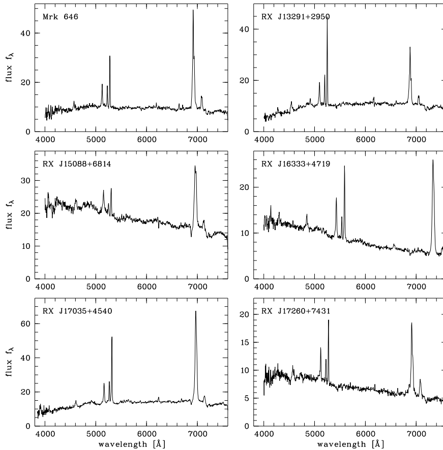
Fig. 1. Optical spectra of the six target galaxies. Fluxes are given as f_\lambda in arbitrary units
