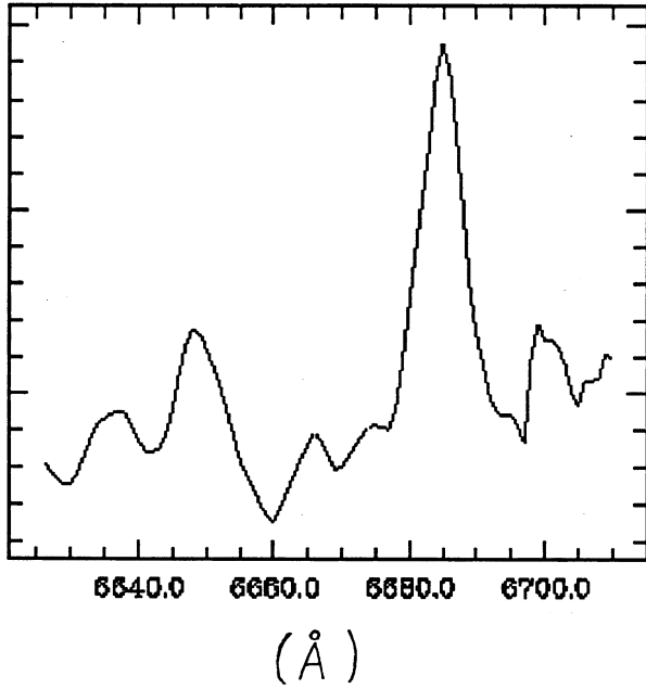
Fig. 2. Nuclear H \alpha spectrum of IC 1689 (vertical scale is arbitrary intensity unit).
