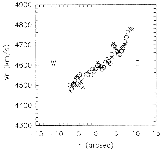
Fig. 5. Emission-line rotation curve of IC 1689 at slit along the major axis of the ring (crosses - H\alpha , circles - [NII]\lambda 6583 ).
