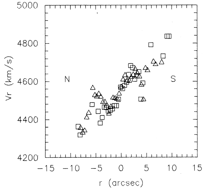
Fig. 3. Absorption-line rotation curve of IC 1689. Different symbols represent heliocentric radial velocities obtained from different spectra.
