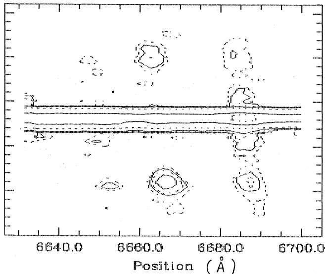
Fig. 4. Spatial structure of H\alpha and [NII] emission lines at slit along the major axis of the ring (continuum influence is suppressed by numerical treatment).
