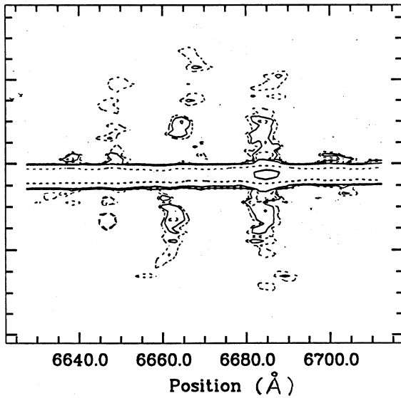
Fig. 6. Spatial structure of H\alpha and [NII] emission lines at slit along the major axis of IC 1689 (continuum influence is suppressed by numerical treatment)
