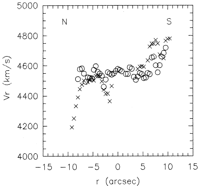
Fig. 7. Emission-line rotation curve at slit along the major axis of IC 1689 (crosses - H\alpha , circles - [NII]\lambda 6583 ).
