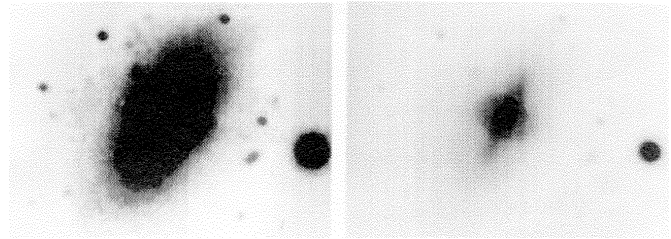
Fig. 1. B -band image of IC 1689 displayed at two different contrasts (in a logarithmic gray scale). North is at the top and east to the left. The entire image field is 60 \times 80 arcsec 2 .
