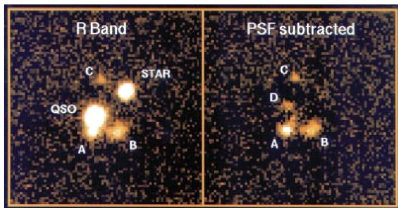
Figure 1: Left: NTT-EMMI R band image of PKS 1610–771 (1200-second exposure, 0.85 \leq seeing). The field is 20'' wide, North is up and East to the left. Right: same image, but a Point Spread Function (PSF) has been subtracted from the quasar and its companion. Three objects (A, B, D) can be seen very close (angle wise) to the QSO. The A–D fuzzy elongation appears perpendicular to the polarisation E vector of the quasar, suggesting their physical relation.
