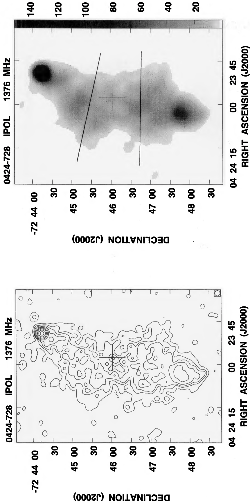
Figure 3. 1376-MHz images of 0424 – 728, as for Fig. 1. Contours are at 1 \text{ mJy beam}^{-1} \times (-2, -0.5, 0.5, 2, 4, 8, 16, 32, 64, 128, 256) , and the beam size is 8 arcsec FWHM. The grey-scale spans the range 0.5\text{--}150 \text{ mJy beam}^{-1} with a beam of 15 arcsec FWHM.
