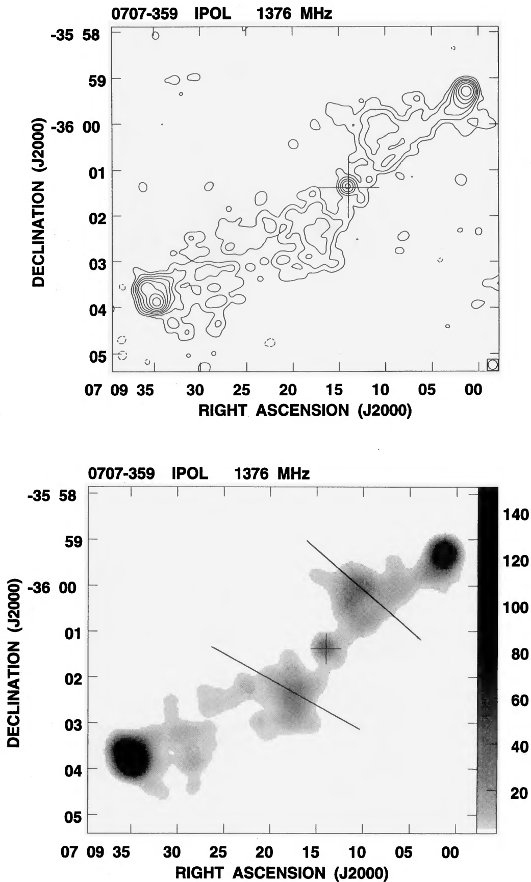
Figure 5. 1376-MHz images of 0707 – 359, as for Fig. 1. Contours are at 1 \text{ mJy beam}^{-1} \times (-1, 1, 3, 8, 16, 32, 64, 128, 256) , and the beam size is 12 arcsec FWHM. The grey-scale spans the range 2\text{--}150 \text{ mJy beam}^{-1} with a beam of 20 arcsec FWHM.
