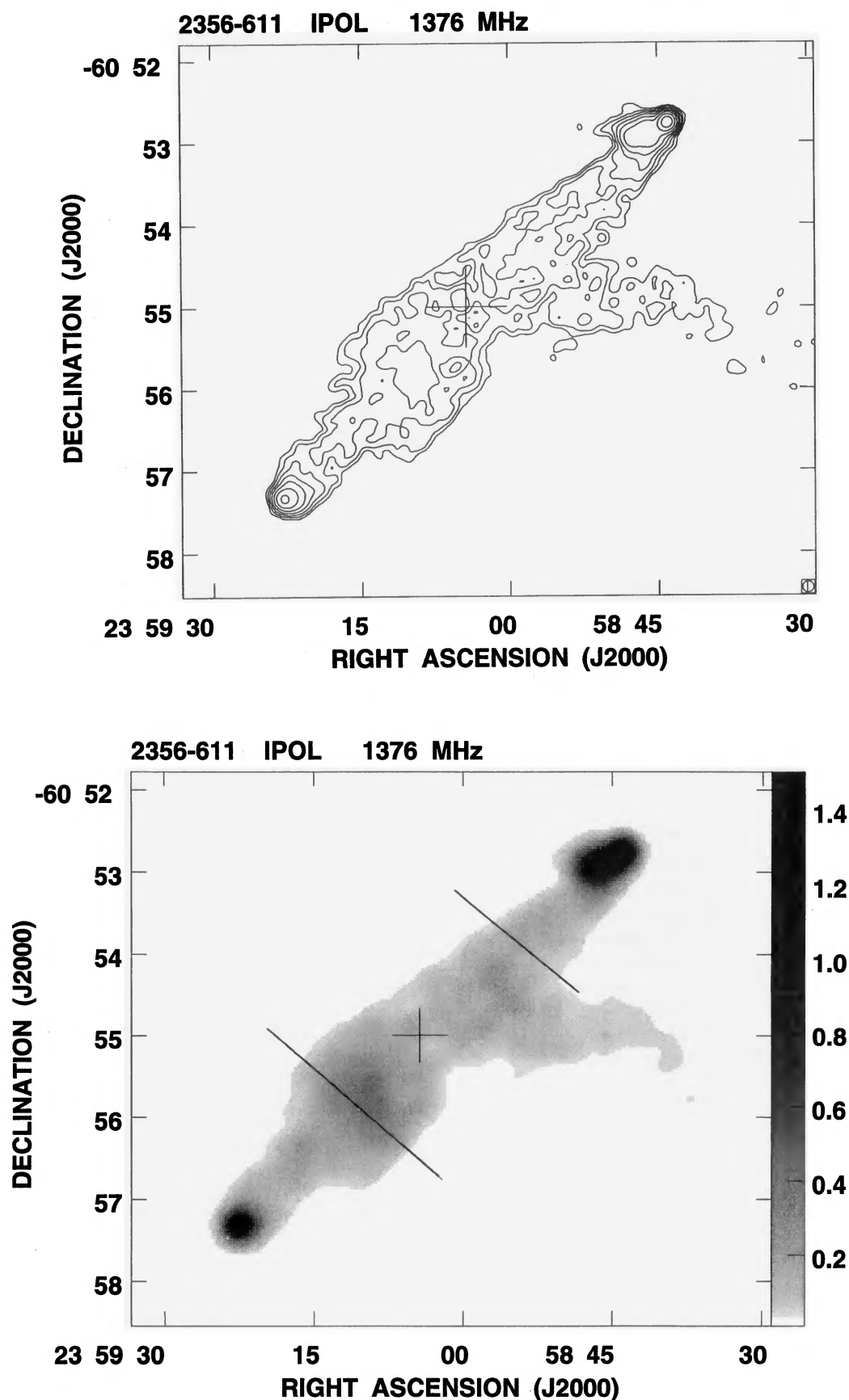
Figure 8. 1376-MHz images of 2356 – 611, as for Fig. 1. Contours are at 10 \text{ mJy beam}^{-1} \times (1, 2, 4, 8, 16, 32, 64, 128, 256) , and the beam size is 8 arcsec FWHM. The grey-scale spans the range 0.015\text{--}1.5 \text{ Jy beam}^{-1} with a beam of 15 arcsec FWHM.
