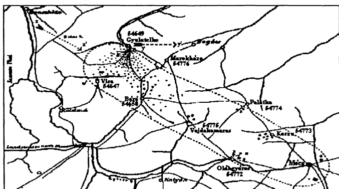
Figure 1: The Mocs meteorite strewnfield, as was originally drawn in Koch's 1882 work. Locations of samples used in this study are marked with the name of the town near where the each fragment was located and the number of each fragment in the collection of the British Museum (Natural History).[3,5]
