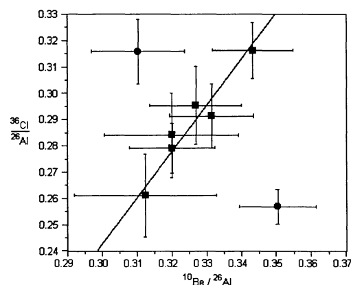
Figure 2: Relationship between ^{10}\text{Be} and ^{36}\text{Cl} (both normalized to ^{26}\text{Al} ) in fragments from the Mocs meteorite strewnfield.
