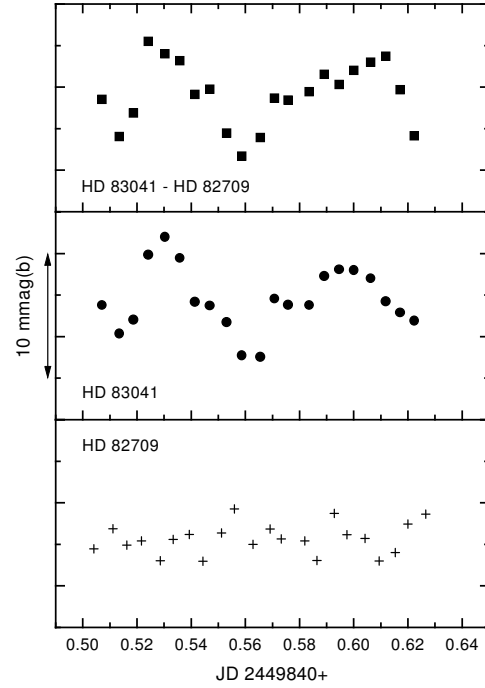
Figure 1. Light curves for HD 83041, HD 82709 and the differential data in Strömberg b
