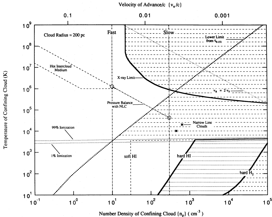
FIG. 5.—Temperature–number density plot for the confining cloud in 2352 + 495. The corresponding velocity of advance derived from the mean hot spot pressure is shown on the top axis. We assume a cloud radius of 200 pc (see text). The upper limit to the optical depth at 151 MHz provides a lower limit to the temperature for an ionized cloud. The upper limit to the X-ray luminosity excludes the portion of the T - n_p plane to the right of the X-ray curve. Also shown are the densities on the fast and slow models, and the hard and soft limits provided by the H I absorption observations and the hard limit provided by CO absorption observations. The region occupied by the narrow line clouds is shown by the two starred points, which correspond to temperatures of 10,000 K and 20,000 K. The region occupied by the “hot intercloud medium” is also indicated. The locus for an external medium in pressure equilibrium with the narrow line clouds is shown by the line marked “Pressure Balance with NLC.” The locus for a medium in which the advance speed is twice the external sound speed is also indicated. The region with horizontal dashes is absolutely excluded, and the region with horizontal dotted lines is excluded for H I but not for H 2 (see text).
