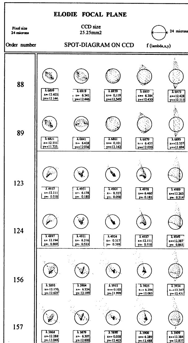
Fig. 3. ELODIE spot-diagrams
