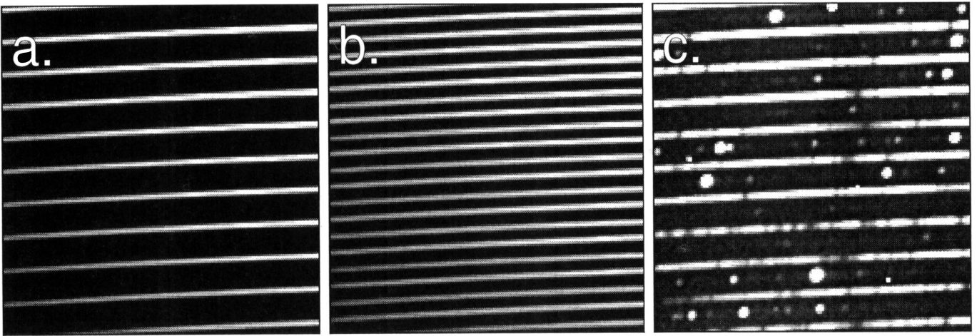
Fig. 6. Small part of the raw image for the three different types of stellar exposure available. a) “star fibre only”, b) star fibre and sky fibre simultaneously illuminated (here by the tungsten lamp), c) “simultaneous thorium”: star on the star hole and the sky hole simultaneously illuminated by the thorium lamp
