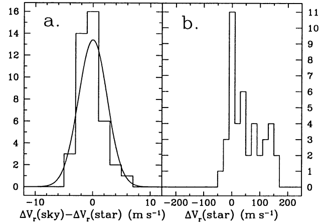
Fig. 19. a) histogram of the velocity shifts between the two way (sky fibre – star fibre). The line is a Gaussian with \sigma = 2.3 \text{ m s}^{-1} . Note that a correction is done to suppress a slight mismatch between the two optical paths: \Delta V_r(\text{sky}) = \Delta V_r(\text{star}) - 0.04 \Delta V_r(\text{star}) + 0.6 ( \Delta V_r is the velocity variation of the spectrograph in units of \text{m s}^{-1} ). b) histogram of the variation of the spectrograph monitor by the star-way during the measurements
