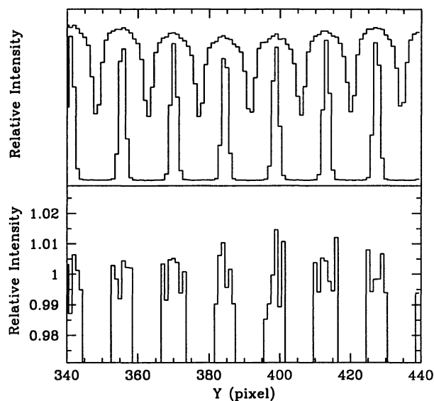
Fig. 13. Top Cross orders tracing at X=500 of a flat-field exposure , superimposed with a localization exposure for comparison. Bottom displays the same crosscut of a flat-field image (corrected from the non-uniform illumination and normalized)
