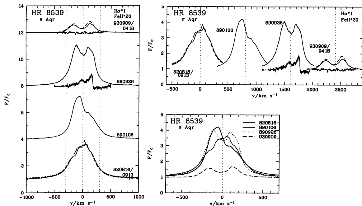
Fig. 78. H\alpha and Fe II profiles for HR 8539
