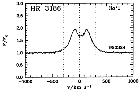
Fig. 41. H \alpha profile for HR 3186
