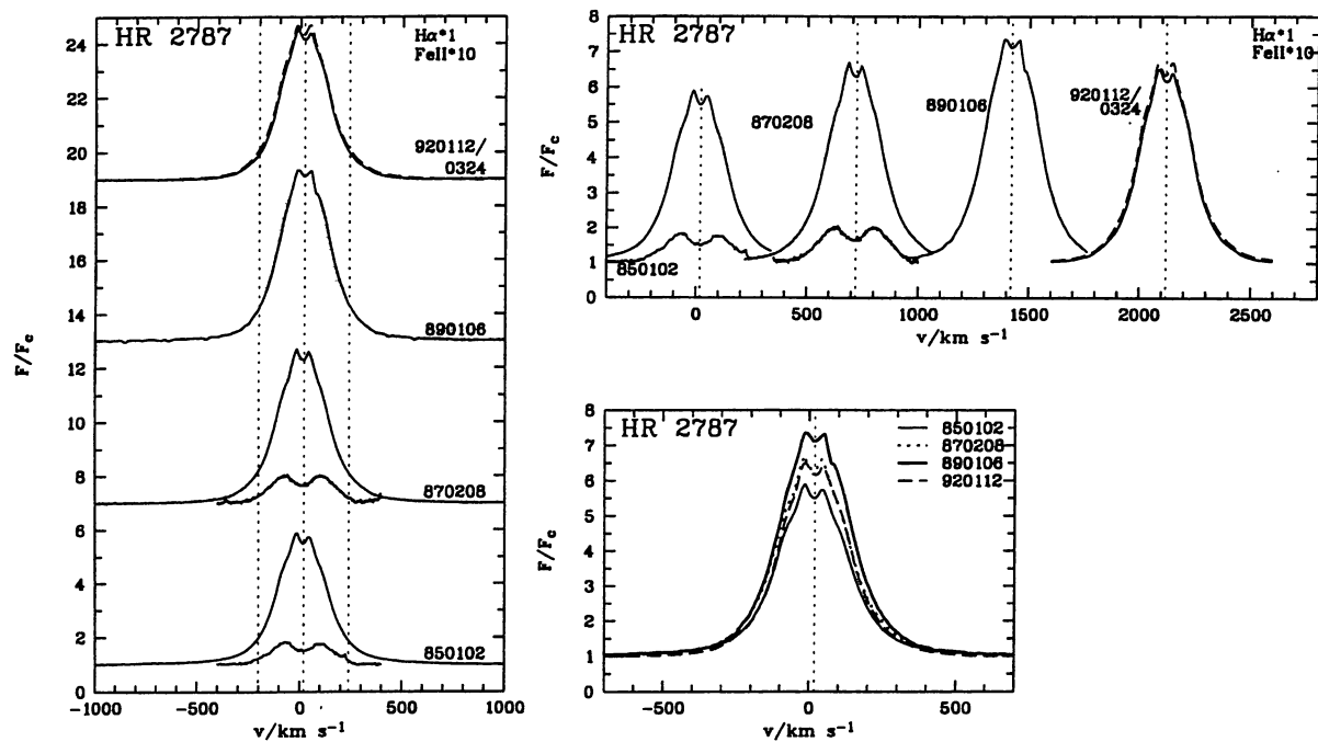
Fig. 33. H \alpha and Fe II profiles for HR 2787
