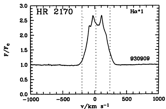
Fig. 21. H \alpha profile for HR 2170
