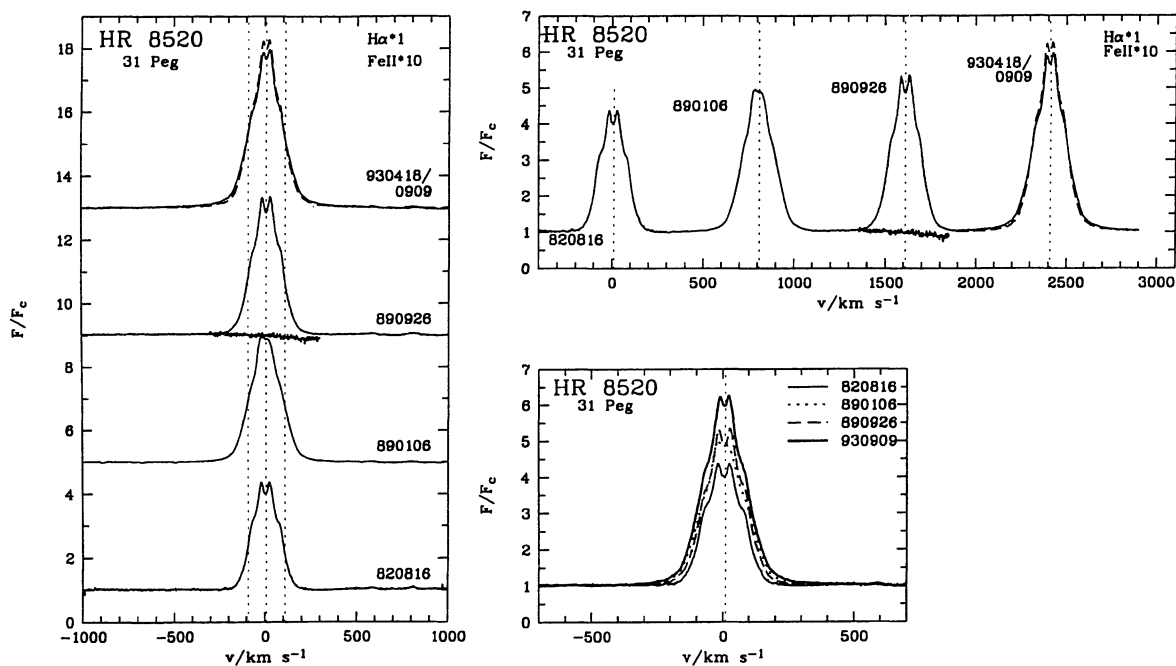
Fig. 77. H\alpha and \lambda 5317 profiles for HR 8520. No trace of Fe II emission is visible. The 890106 profile from SI92 is not fully resolved
