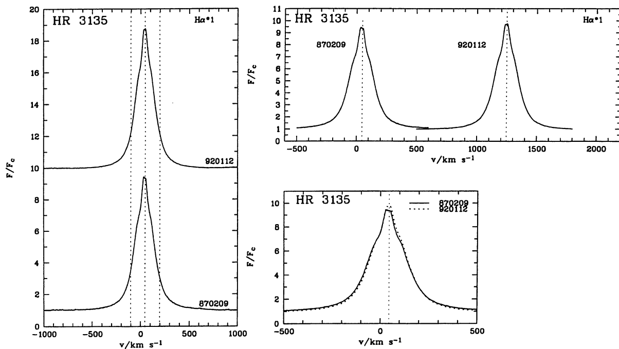
Fig. 40. H\alpha profiles for HR 3135
