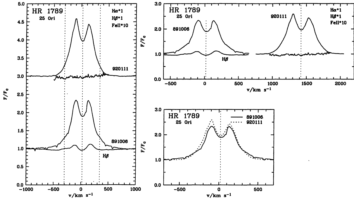
Fig. 15. H\alpha , H\beta and \lambda 5317 profiles for HR 1789 (no emission visible in Fe\ II )
