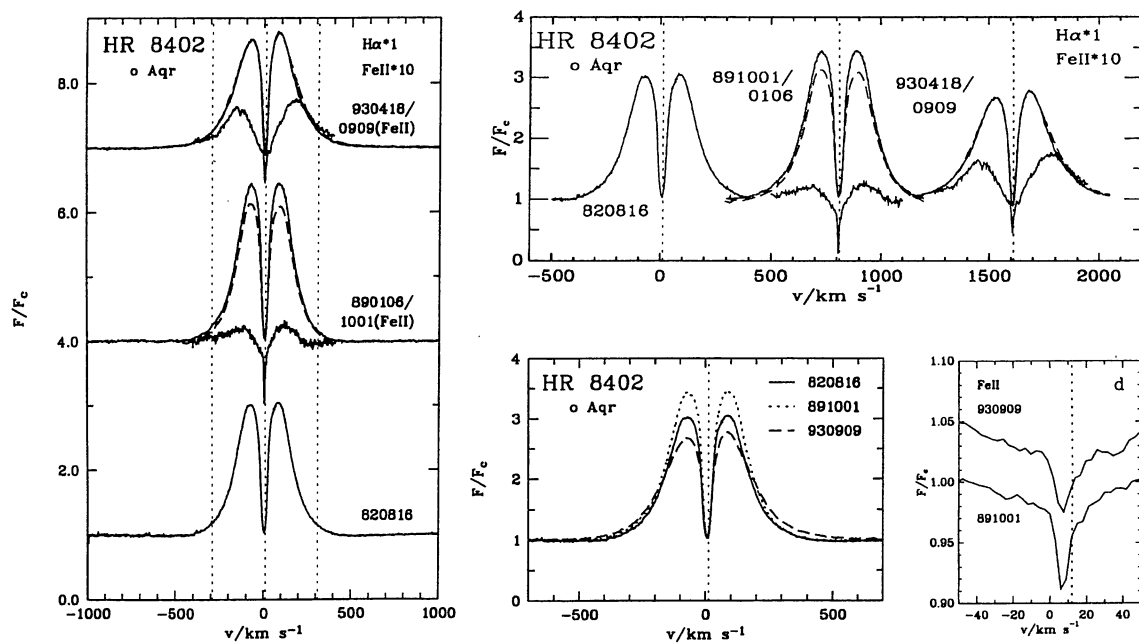
Fig. 75. H\alpha and Fe II profiles for HR 8402. Panel d shows a blow-up of the extremely narrow Fe II lines. Note that in panels a and b, the depth of the Fe II lines is affected by the expansion
