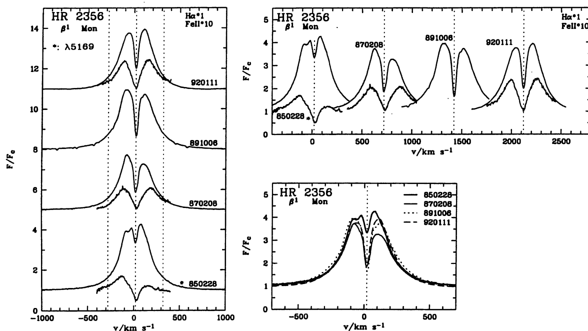
Fig. 26. H \alpha and Fe II profiles for HR 2356. In 1985, the Fe II \lambda 5169 line has been measured instead of \lambda 5317 (marked by an asterisk)
