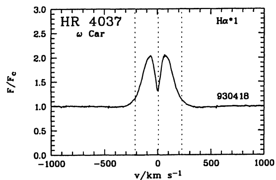
Fig. 47. H\alpha profile for HR 4037
