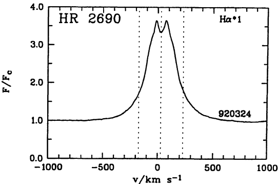
Fig. 30. H \alpha profile for HR 2690
