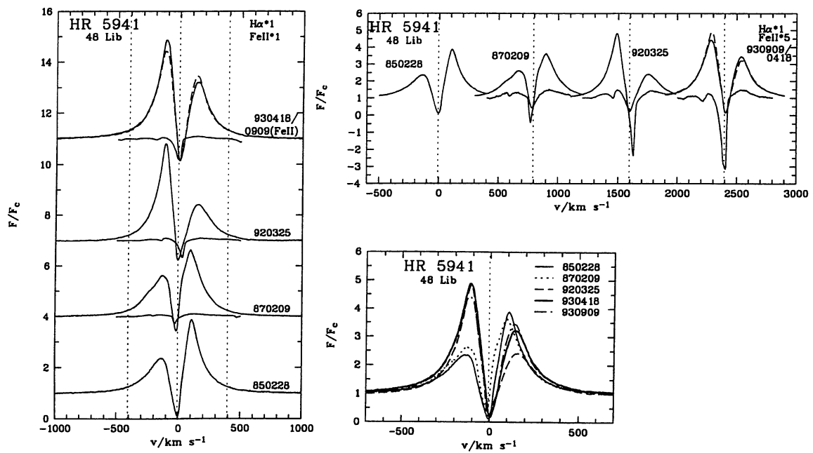
Fig. 63. H\alpha and Fe II profiles for HR 5941. Note that the scaling for Fe II lines is different in panels a and b, and that the depth of the Fe II troughs in panel b is affected by the expansion
