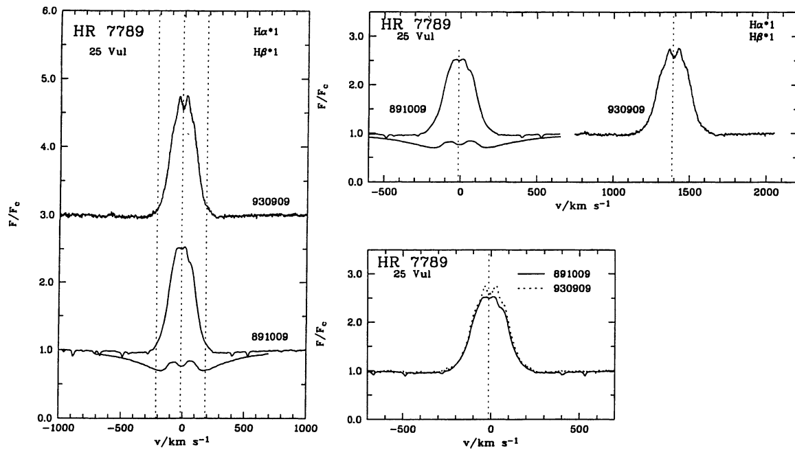
Fig. 73. H\alpha and H\beta profiles for HR 7789. Note that the 891009 profiles (from Sl92) are not fully resolved
