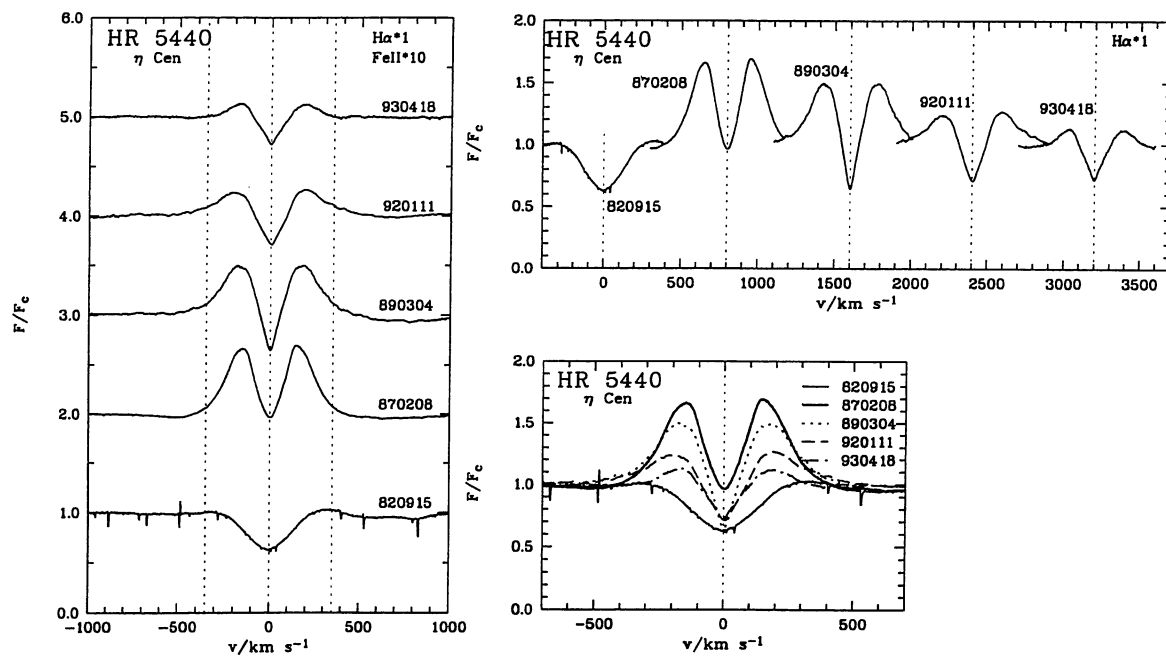
Fig. 58. H \alpha profiles for HR 5440
