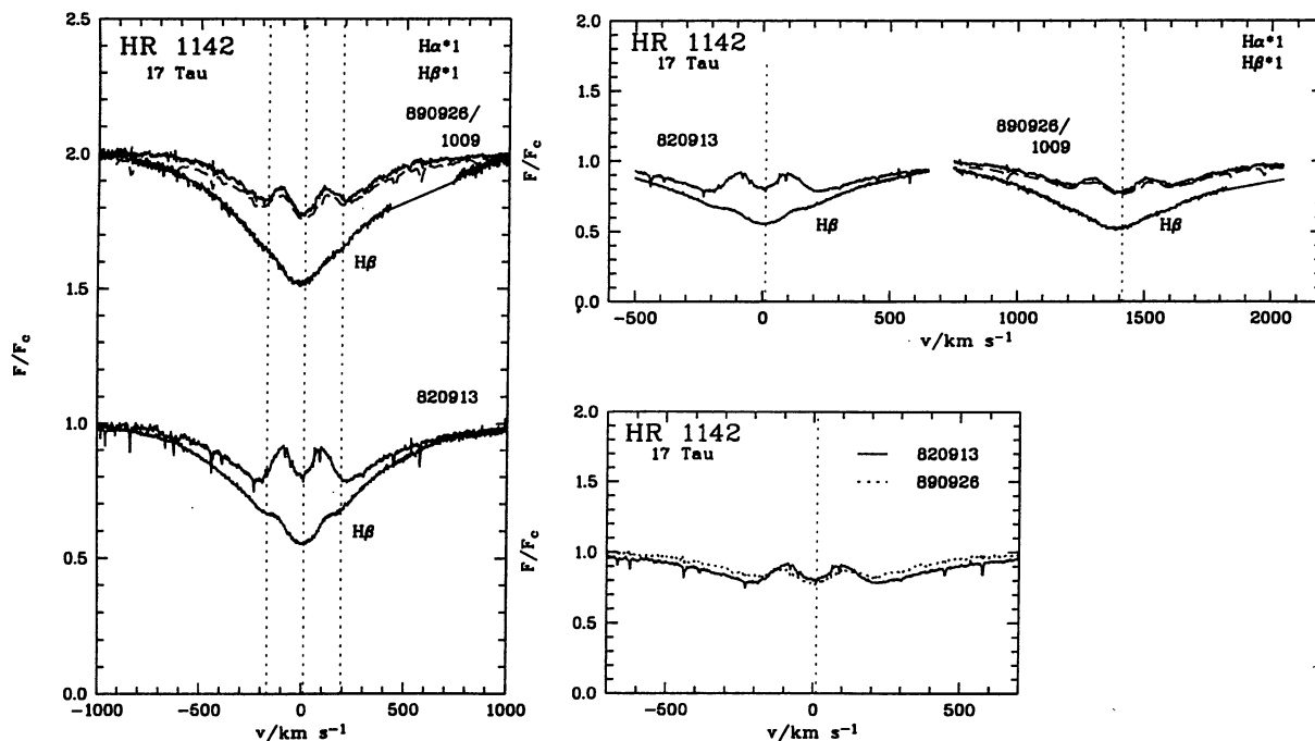
Fig. 6. Same as Fig. 5, for HR 1142 = 17 Tau. Here, and in all following plots, the convention is that profiles plotted as broken line have been measured on the date given behind the slash (here: 891009 in a ))
