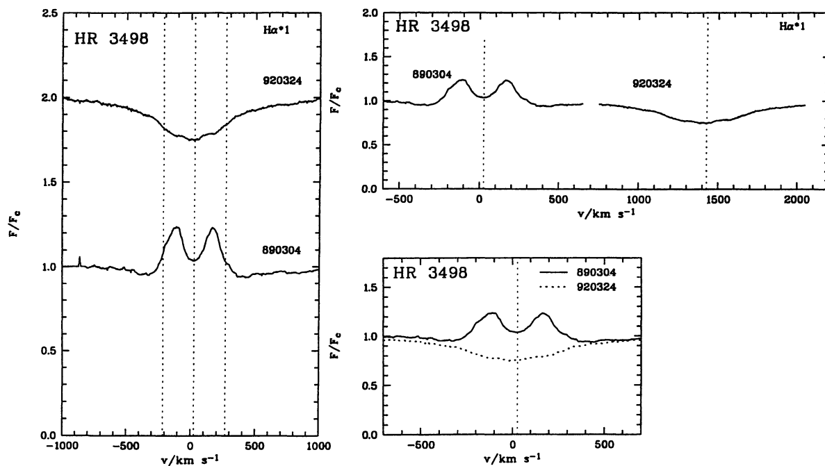
Fig. 43. H \alpha profiles for HR 3498
