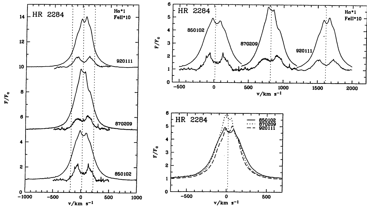
Fig. 24. H \alpha and Fe II profiles for HR 2284
