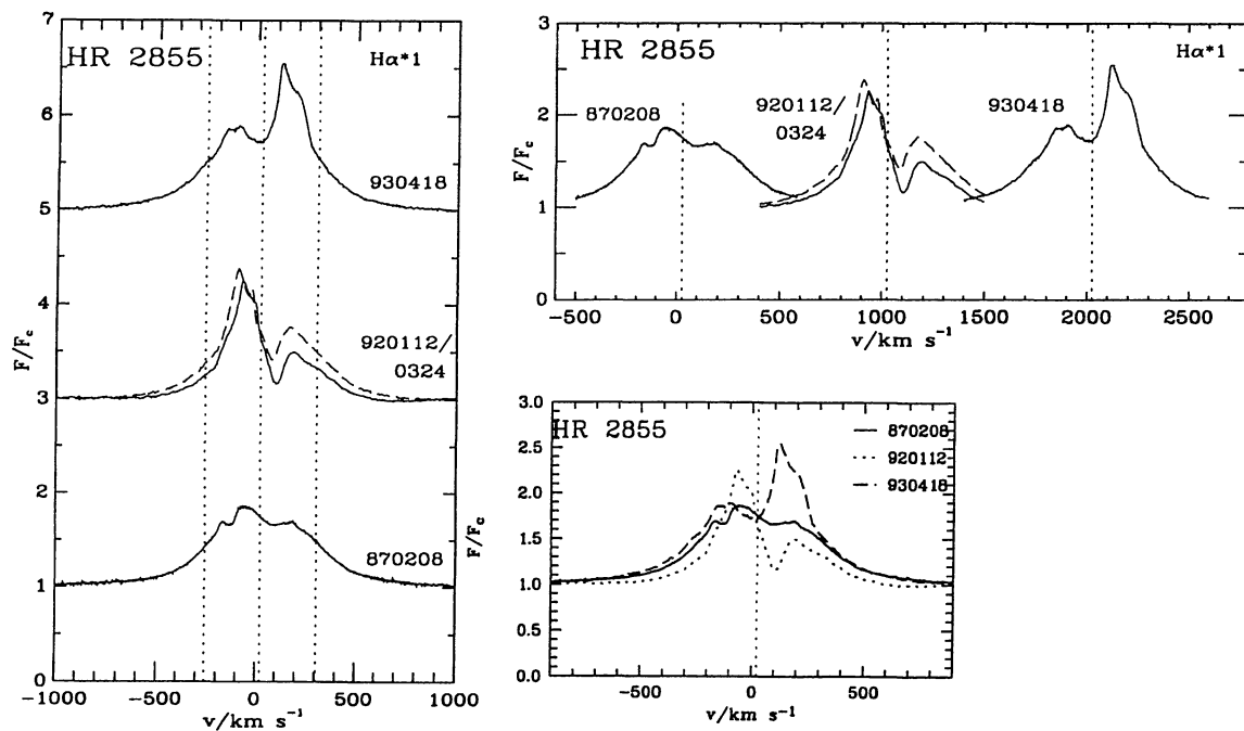
Fig. 36. H\alpha profiles for HR 2855 (Fe II emission was present in 1992, but profile has been lost)
