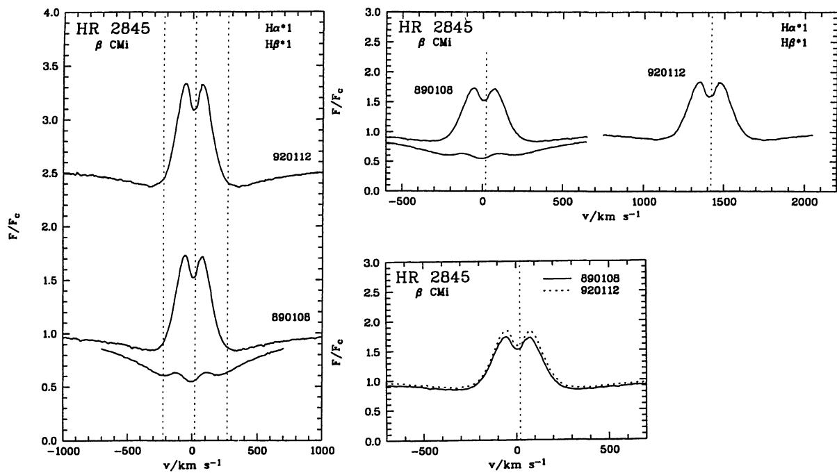
Fig. 35. H\alpha and H\beta profiles for HR 2845
