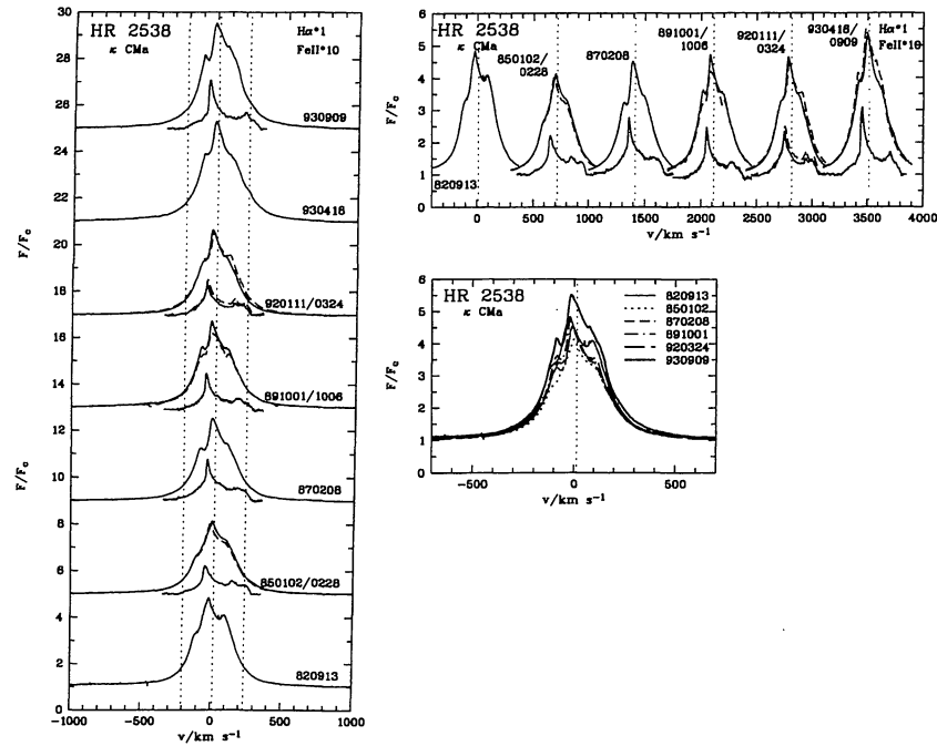
Fig. 28. H \alpha and Fe II profiles for HR 2538
