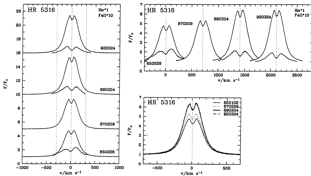
Fig. 57. H \alpha and Fe II profiles for HR 5316
