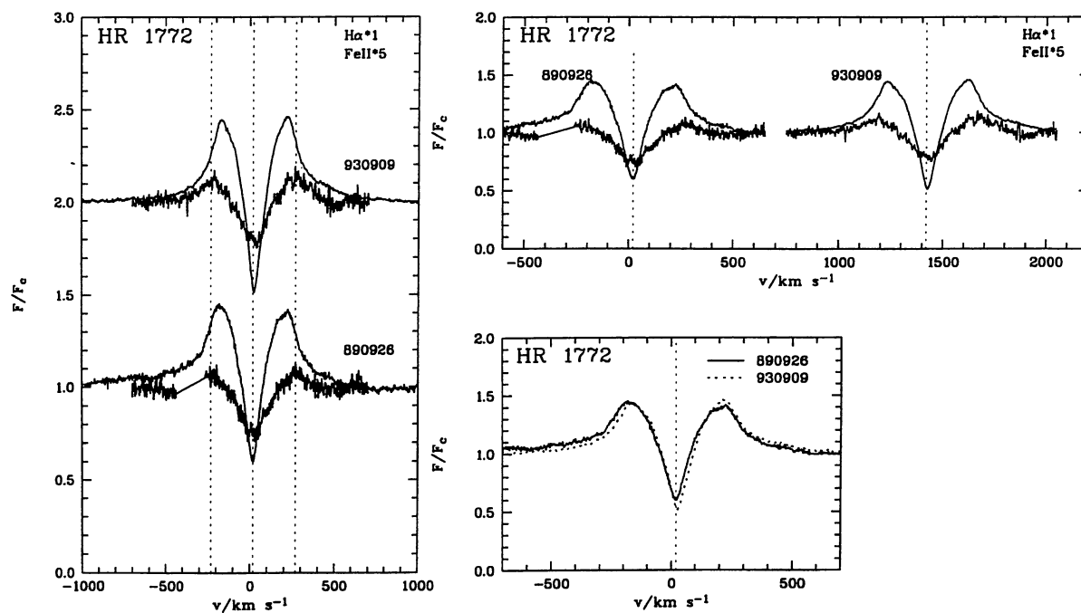
Fig. 14. H\alpha and Fe\ II profiles for HR 1772
