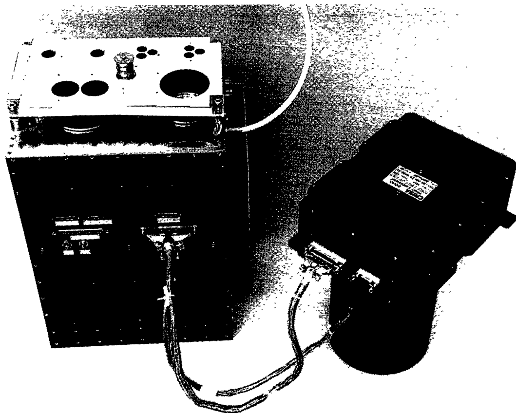
Fig. 1. VIRGO sensor package (left-hand side, outside dimensions 392×293×230 mm, weight 13.0 kg) and power supply (right-hand side, outside dimensions 250×204× 90 mm, weight 1.5 kg). The SP will be mounted at the feet which end at half-way between the top and the bottom; this is also the reason why the PS is put on a stand for the picture, the height of which corresponds to its mounting level. The instrument apertures (clockwise from left upper corner of SP) are for 2 PMO6-V radiometer, 2 SPM, LOI and DIARAD.
