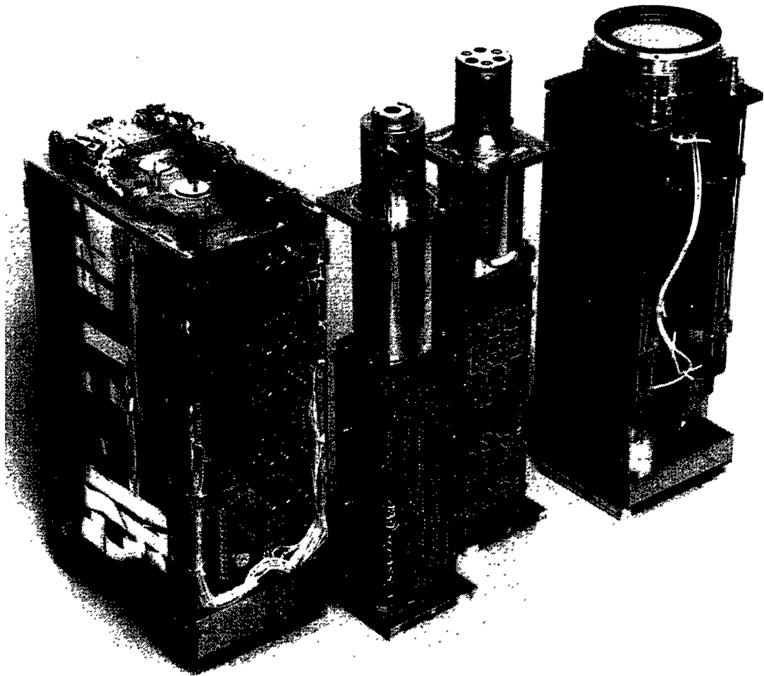
Fig. 2. The four types of instrument in the VIRGO SP (from left): DIARAD, PMO6-V, SPM and LOI.
