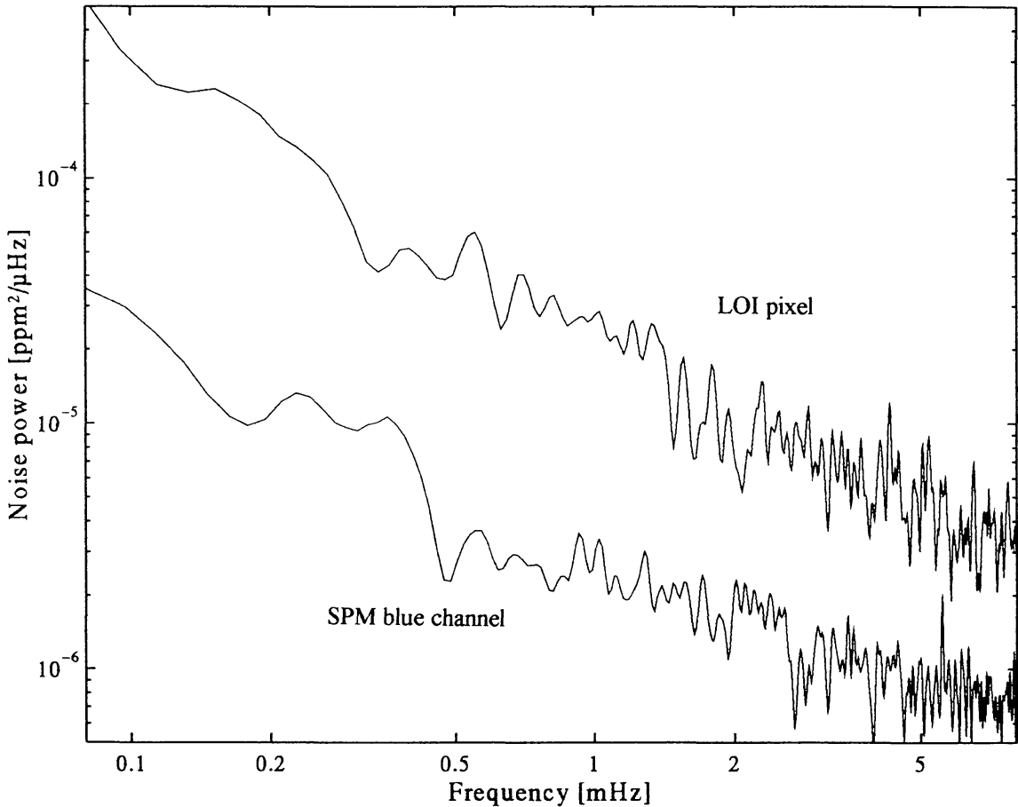
Fig. 6. Power spectral density of the dark-current noise of the SPM blue channel (lower curve) and a LOI pixel (upper curve) calculated from time series of 68 and 45 h respectively. In the 5-minute range the noise of the SPM is about 5 \times 10^5 times smaller than the noise between the p-mode lines of IPHIR ( \approx 0.5 \text{ ppm}^2 \mu\text{Hz}^{-1} ) and of the LOI pixel 1.2 \times 10^6 times smaller than the noise expected for a 12th of the solar disk (12 times the noise power of the full disk).
