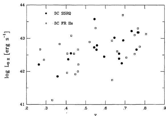
FIG. 7—The [O II] emission-line luminosity for quasars (filled circles) and powerful (FR II) radio galaxies (open squares) in the 3CR sample, plotted vs. redshift to allow comparisons at similar radio luminosity (which is well correlated with redshift in a radio-flux-limited sample) and/or observed wavelength of [O II]. The narrow-emission-line luminosities of radio galaxies and quasars, which should be unaffected by obscuration or relativistic beaming, span the same values over the full redshift range. (Data from Hes et al. 1993.)
