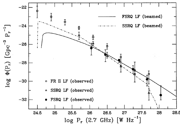
FIG. 14—Local differential radio luminosity functions for high-luminosity radio sources: flat-spectrum radio quasars (filled circles), steep-spectrum radio quasars (open triangles), and FR II galaxies (open squares). The error bars represent the sum in quadrature of the 1\sigma Poisson errors (Gehrels 1986) and the variations of the number density associated with a 1\sigma change in the evolutionary parameter \tau (see Padovani and Urry 1992 for details). The luminosity functions of FR IIs and SSRQ have similar slopes and extend to the same luminosity at the bright end, although the FR IIs extend a decade lower at the faint end. The FSRQ luminosity function is distinctly flatter and extends to higher luminosities. This agrees well with the predictions of a beaming model calculated for FSRQ (solid line) and SSRQ (dot-dashed line); see Sec. 6.1.3 (Table 3) for details of the model parameters.
