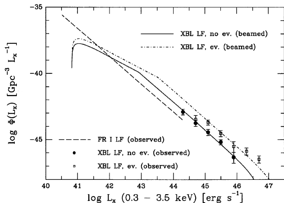
FIG. 16—The local differential X-ray luminosity functions of low-luminosity radio-loud AGN. The observed LF of FR I galaxies is represented by a broken power law ( dashed line ). The observed LFs for the EMSS XBL sample (no evolution: filled circles ; anti-evolution: open squares ) are fitted by beaming models for the non-evolving case ( solid line ) and the anti-evolving case ( dash-dotted line ); data and evolution estimate from Wolter et al. (1994). Error bars correspond to 1\sigma Poisson errors (Gehrels 1986).
