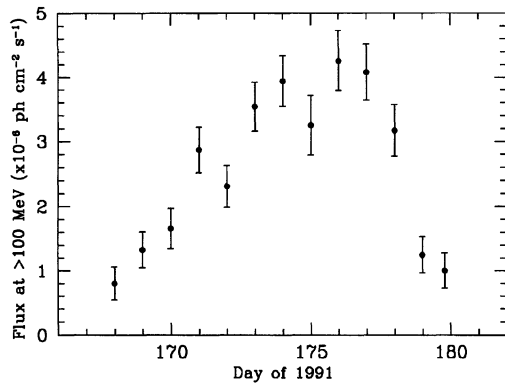
FIG. 5—Gamma-ray light curve of the superluminal quasar 3C 279 during the bright outburst in June 1991 (Kniffen et al. 1993). The combination of rapid variability and high gamma-ray luminosity strongly suggests the emission is relativistically beamed. (Copyright American Astronomical Society, reproduced with permission.)
