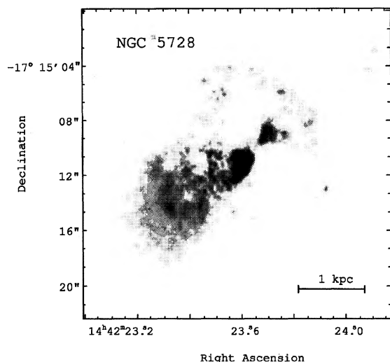
FIG. 3— HST WFPC image of the nearby Seyfert 2 galaxy NGC 5728 taken in the light of [O III] with resolution 0.1 arcsec (Wilson et al. 1993). The biconical structure suggests that a hidden nuclear source with quasar-like ultraviolet luminosity is photoionizing gas in the narrow-line region. (Copyright American Astronomical Society, reprinted with permission.)
