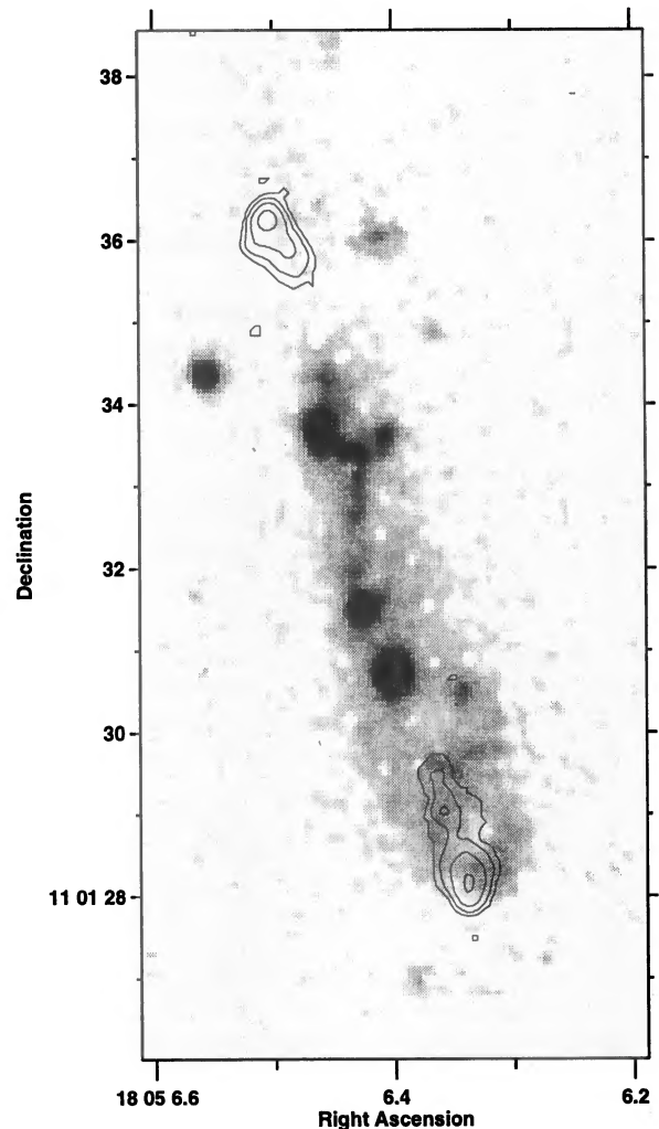
Figure 1. 3C 368: the image is the sum of both filters of the WFPC2 observations. The VLA data are superimposed, the contour levels being at (1, 4, 16, 64) \times 1.18 \times 10^{-4} Jy beam ^{-1} .
