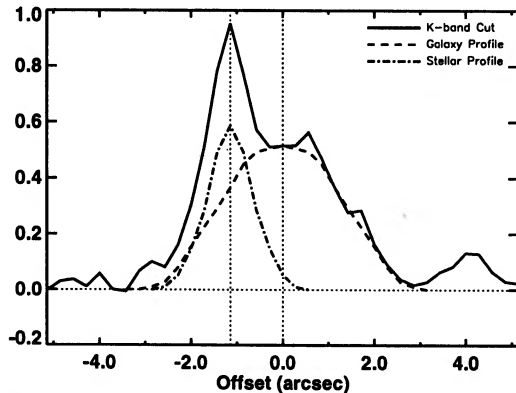
Figure 2. A cut along the axis of 3C 368 in the 2.2- \mu\text{m} K wave-band. The y-axis shows intensity relative to the peak intensity, and error bars are \pm 0.003 . The intensity distribution has been decomposed into the M star (dot-dash line) and the residual parent galaxy (dashed line). The centre of the galaxy lies just over 1 arcsec north of the M star.
