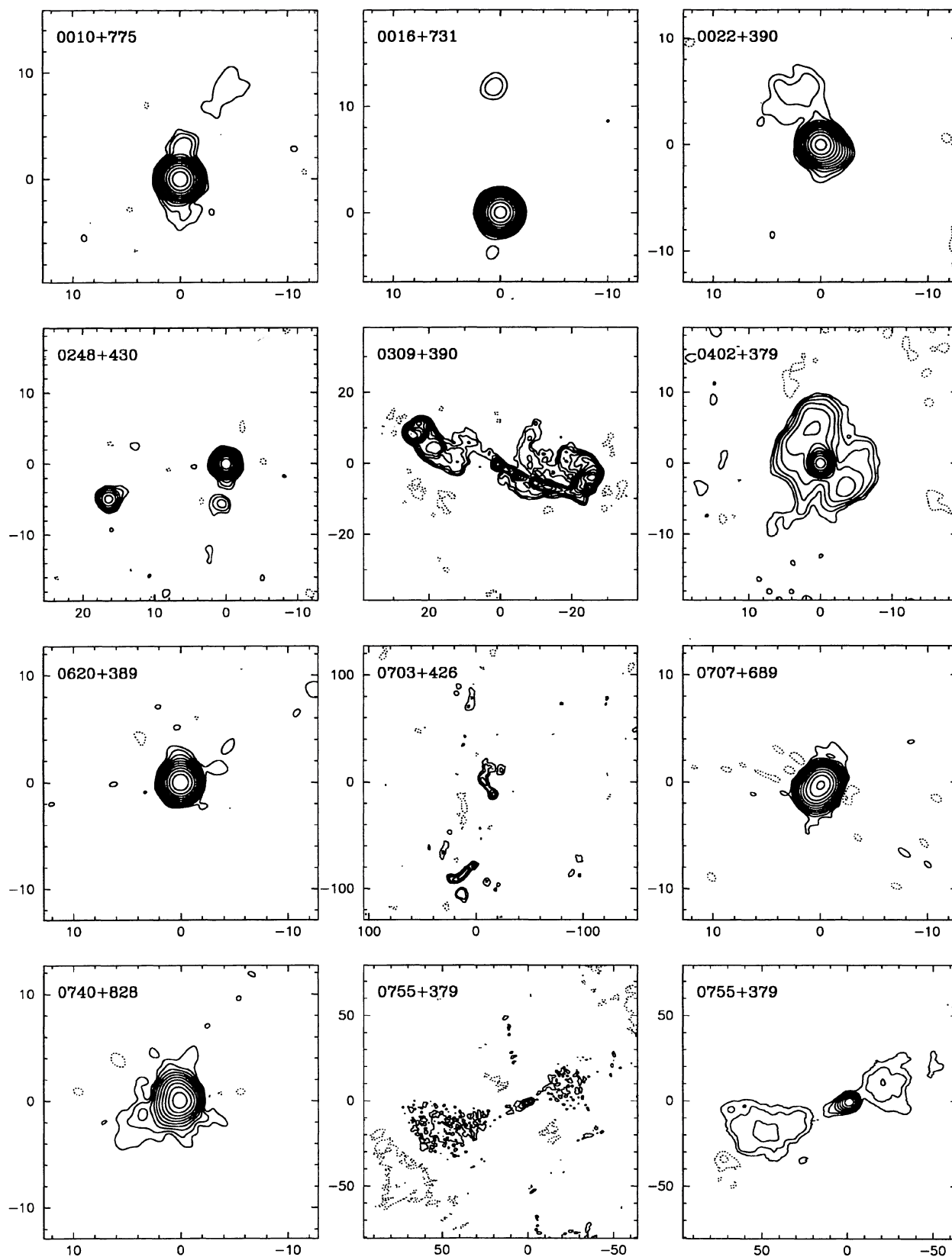
FIG. 6.—The 1.4 GHz VLA maps of 64 objects with extended structure. The naturally weighted map is shown for each object. Unless noted otherwise in Table 6, logarithmic contour levels are used in all maps, drawn at -2, -1, 1, 2, 4, 8, 16, \dots, 1024 \times 3 \sigma (where \sigma is the rms noise measured in a blank region of the map), and the maps are restored with a circular Gaussian beam of FWHM 1''.5 . For 0755+379 and 0827+378, the map restored with a larger beam is also shown. The peak intensity and rms noise are given in Table 6. The angular scale is marked in arcseconds. FITS images corresponding to the maps presented in Fig. 6 are published in the AAS CD-ROM Series, Vol. 5.
