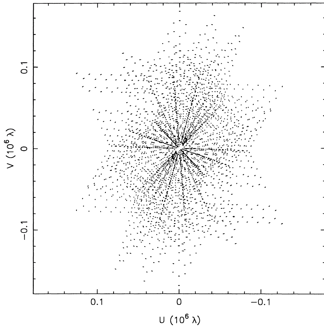
FIG. 5.—Typical uv coverage for VLA observations: \delta \approx 41^\circ (1242+410 observed on 1992 November 5 at 1.365 GHz).
