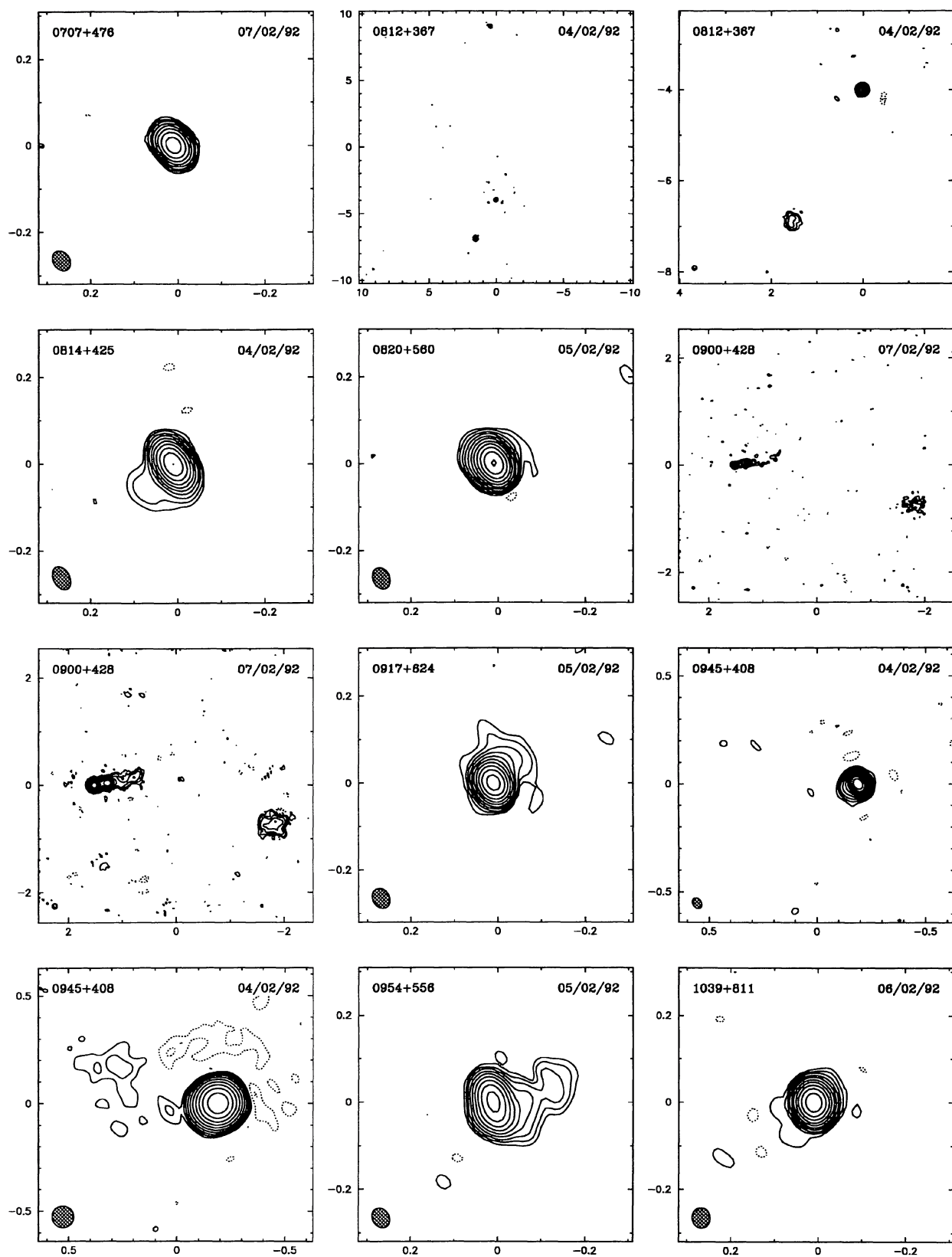
FIG. 4.—The 5 GHz MERLIN uniformly weighted maps of 20 objects. Logarithmic contour levels are used in all maps, at -2, -1, 1, 2, 4, 8, 16, \dots, 1024 \times 3 \sigma (where \sigma is the rms noise measured in a blank region of the map). The FWHM contour of the elliptical Gaussian restoring beam is shown hatched in the lower left-hand corner. For 0812+367, 0900+428, 0945+408, and 1800+440, which have large angular sizes, the naturally weighted map restored with a circular beam of FWHM 100 mas is also shown. In addition, an enlarged map of 0812+367 is presented to show the central and southern components in more detail. The peak intensity, rms noise, and parameters of the restoring beam are listed in Table 5. The angular scale is marked in arcseconds. FITS images corresponding to the maps presented in Fig. 4 are published in the AAS CD-ROM Series, Vol. 5.
