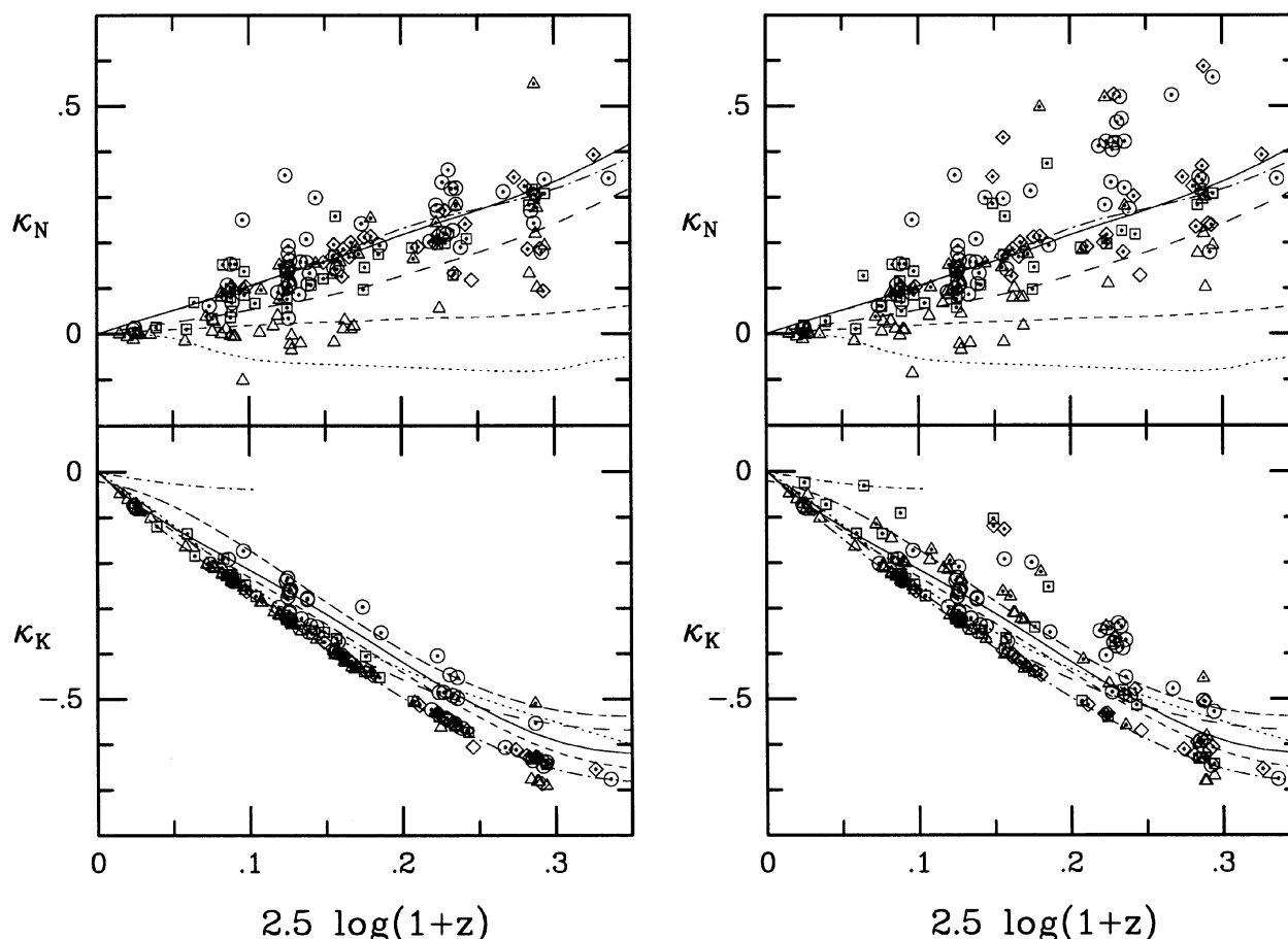
FIG. 9. The \kappa -corrections for the N and K bands as determined from the free two-star model are plotted as a function of redshift. Each point represents a galaxy in our sample at its observed redshift. Galaxies with >20\% saturation in any band have been excluded from the plot. The left-hand panel is for the (adopted) two-star model without K and M dwarfs. The right-hand panel shows the effect of allowing the model to choose K and M dwarfs. The symbols and curves are the same as in Fig. 8, with the addition of two additional curves for the K band, in descending order: (1) Mobasher et al. 's (1986) semi-empirically derived \kappa -correction (small-dash-dotted line); (2) an elliptical galaxy spectrum as reported by Eisenhardt & Lebofsky (1987, long-dash-dotted line). These two curves lie above the previous four curves.
