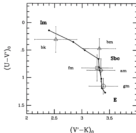
FIG. 14. The distribution of mean colors for rest-frame U-V' and V'-K for different spectral types and Hubble types. Error bars represent the standard deviation of colors within each spectral type. Mean colors for Hubble types are derived as discussed in the text. Mean colors for spectral types are listed in Table 4.
