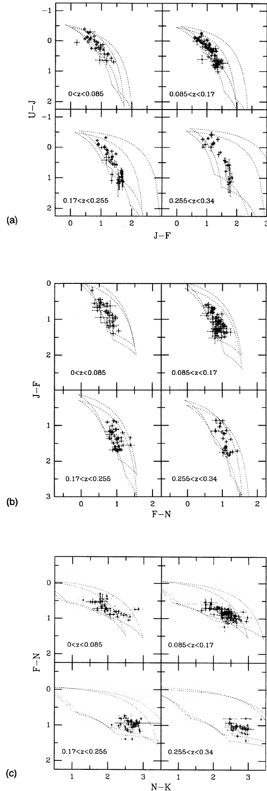
FIG. 2. The observed multicolor distribution of our galaxy sample is displayed again as in Fig. 1. Here, the dotted lines represent the boundaries of the color space attainable by all positive linear combinations of four fixed stellar types (see text): BV, G2V, K3III, M2III. The dotted lines are drawn at the redshifts corresponding to the bin boundaries.
