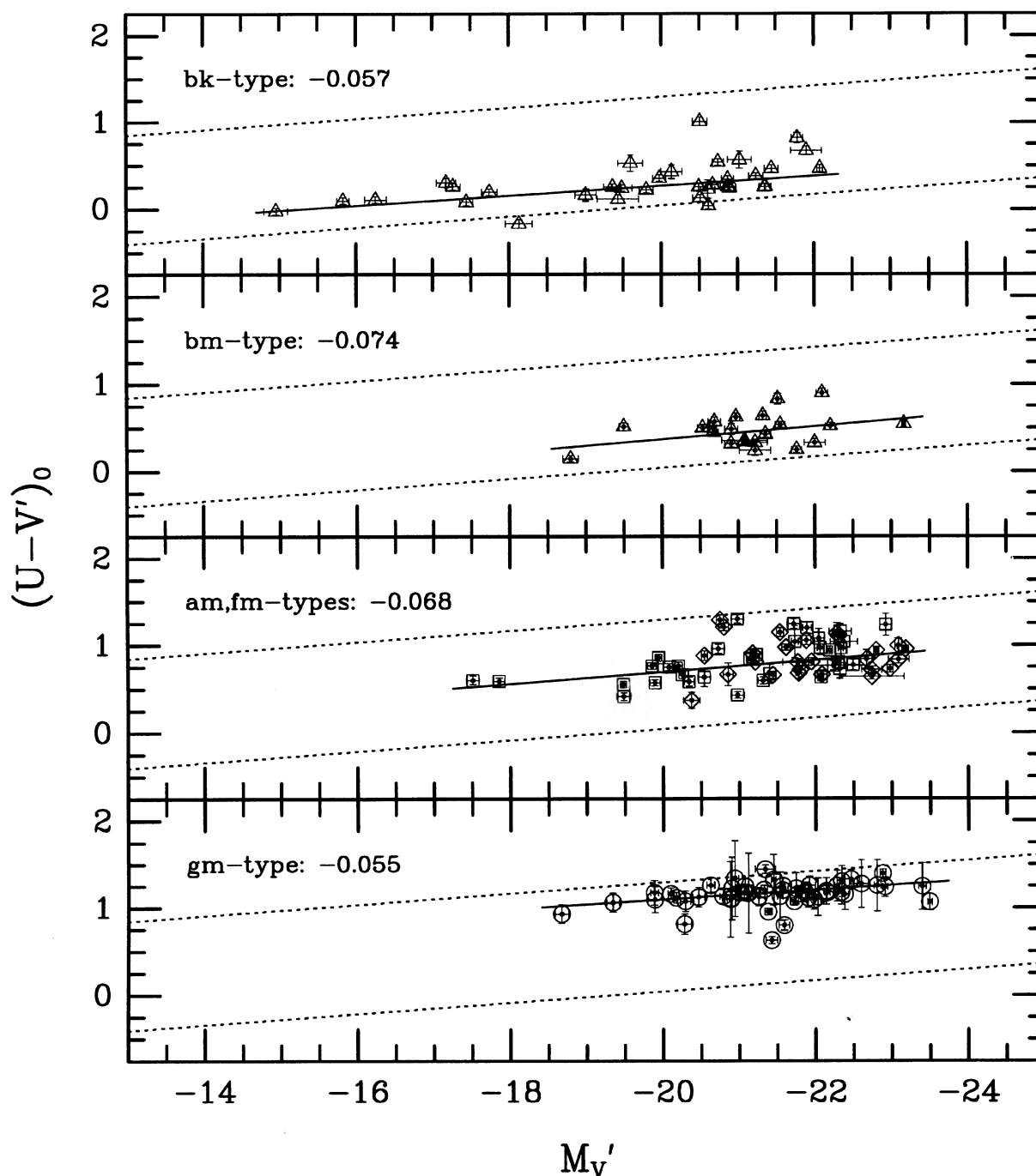
FIG. 16. The color–luminosity effect is shown for each spectral type for rest-frame U-V' vs M_{V'} . Linear regressions, described in the text, are shown as solid lines, and their slopes are indicated next to the spectral type. Dotted lines are drawn at a separation of 1.25 mag with slopes equal to the average for all spectral types. The zero-points of these lines are set arbitrarily to bracket the combined distribution of all spectral types. Error bars represent estimated photometric errors.
