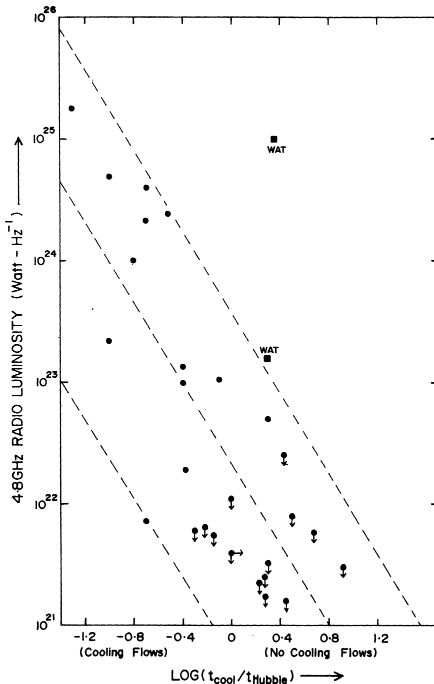
Figure 3. Plot of the radio luminosity of cD galaxies versus cooling time of the intracluster gas in the clusters. Radio luminosity at 4.8 GHz (in \text{WHz}^{-1} ) is plotted against the log normalised cooling time ( t_{\text{cool}}/t_{\text{Hubble}} ) for the intracluster medium in the cluster core. Upper limits on radio luminosities are indicated by arrows. The central dashed line is the best fitting regression line described in the text and the other two dashed lines represent the upper and lower envelopes. Two wide-angled-tailed (WAT) radio sources are shown by a filled square symbol.
