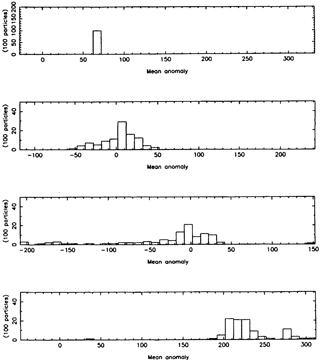
FIG. 2. Dust trail formed from the Taurid Complex progenitor after the presumed release of Comet P/Encke. The constraint that to be released from the resonant progenitor Encke must be in the resonant zone means that the event must have occurred between about 1772 and the Encke discovery date of 1786. Interestingly the previous favourable chance for Encke's discovery before 1786 would have been during the 1772 apparition (see Kronk 1984). Our computer models of the trail give better fits to the IRAS observations for starting dates nearer 1772. In the model shown here the particles separated from the parent in 1773 (first plot) with isotropic ejection velocities up to 15 \text{ m s}^{-1} and the perturbative effects of Jupiter, Earth and Venus have been included. In each plot the mean anomaly M is positioned so that the resonance centre is at the centre of the plot. Thus initially the progenitor, Encke and dust particles are 80\text{--}90^\circ behind the resonance centre and so at the back of the resonant zone. In the second and third plots (50 and 100 yr later) the motion forward through the resonance is shown. In the final plot M is shown at the time of the IRAS observations (mid-1983), when this model progenitor has M = 215^\circ . The brightest part of the observed trail is between M = 200 and 260^\circ . The resonant zone (at the centre of which we believe the meteoroidal swarm is concentrated) is between M = 40 and 220^\circ so that the progenitor is near the front of the resonant zone, at the extreme of its oscillation.
