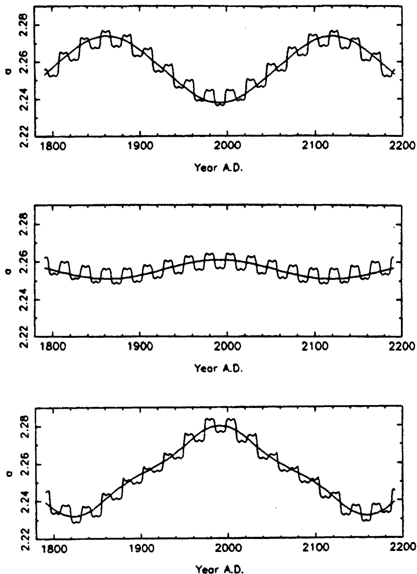
FIG. A1. Orbital behaviour of three 7:2 resonant Taurids (with different libration amplitudes) as given by smoothed analytic theory and by numerical integration.
